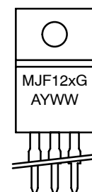
TO-220 CASE 221D-02 STYLE 2
