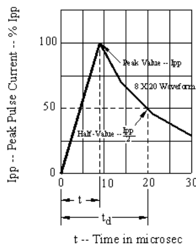
FIGURE 2 Pulse Wave Form
