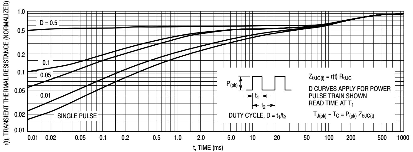
Figure 16. Thermal Response
