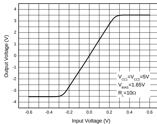
Figure 5. Tracking Driver Characteristics (Note 6)
