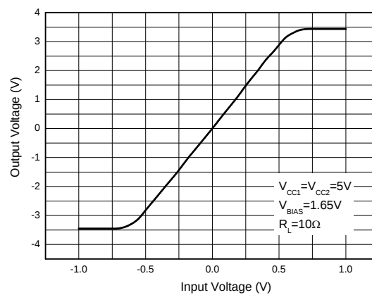
Figure 7. Spindle Driver Characteristics (Note 6)
