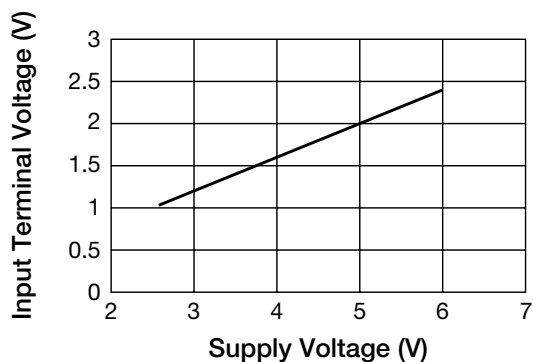
Input Terminal Voltage vs Supply Voltage
