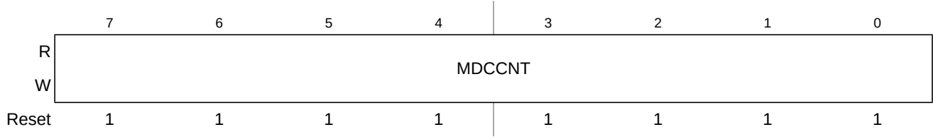
Figure 10-7. Modulus Down-Counter Count Register Low (MDCCNT)
