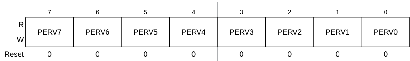
Figure 4-53. Port V Pull Device Enable Register (PERV)
