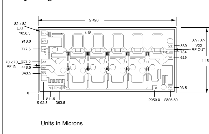
Chip Diagram
