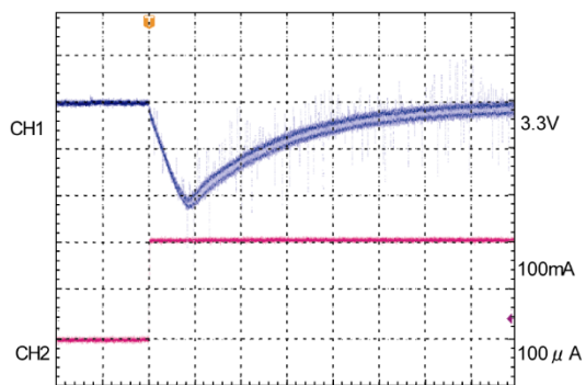
200 \mu sec/div CH1: V_{OUT1} , AC-COUPLED, 50mV/div CH2: I_{OUT1} , 50mA/div
