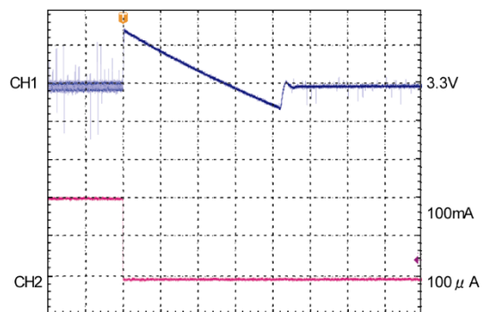
10msec/div CH1: V_{OUT1} , AC-COUPLED, 50mV/div CH2: I_{OUT1} , 50mA/div
