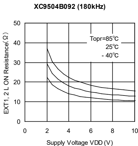
(19) EXT1, 2 Low ON Resistance vs. Supply Voltage
