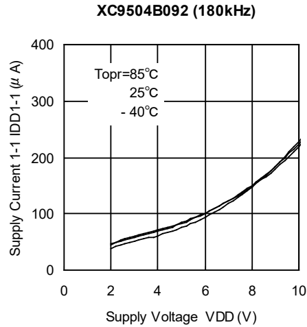
(9) Supply Current vs. Supply Voltage
