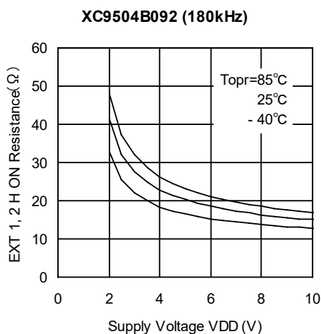
(18) EXT1, 2 High ON Resistance vs. Supply Voltage
