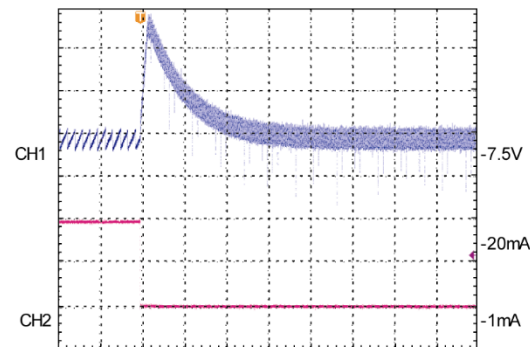
400 \mu sec/div CH1: V_{OUT2} , AC-COUPLED, 20mV/div CH2: I_{OUT2} , 10mA/div
