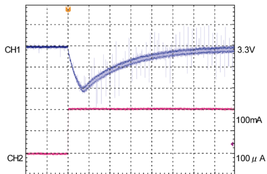
200 \mu sec/div CH1: V_{OUT1} , AC-COUPLED, 50mV/div CH2: I_{OUT1} , 50mA/div
