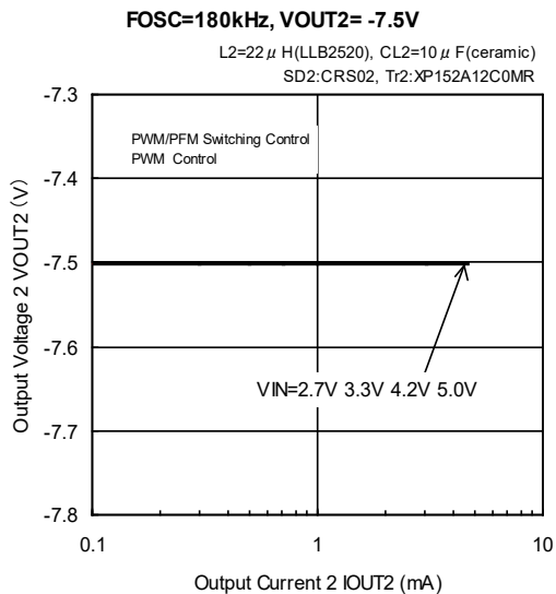
(4) Output Voltage vs. Output Current
