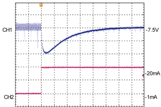
200 \mu sec/div CH1: V_{OUT2} , AC-COUPLED, 20mV/div CH2: I_{OUT2} , 10mA/div
