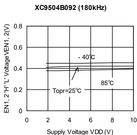
(15) EN1, 2 'H'L' Voltage vs. Supply Voltage
