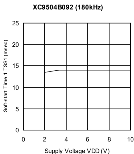
(17) Soft-Start Time 1 vs. Supply Voltage
