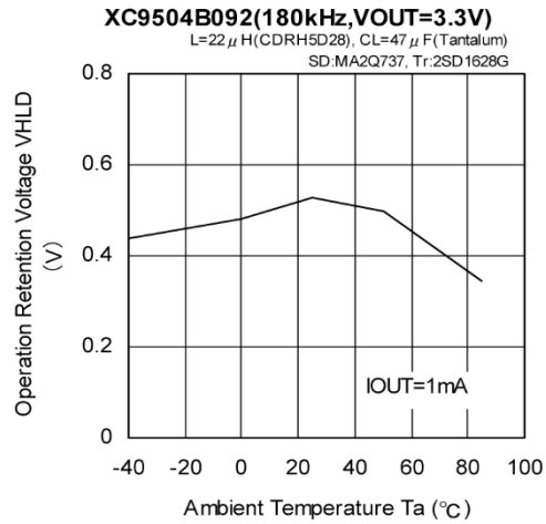
(21) Operation Retention Voltage vs. Ambient Temperature
