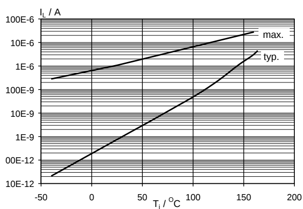
Fig.11. Typical off-state leakage current. I_L = f(T_J) ; conditions V_{BL} = 16\text{ V} = V_{BG} , V_{IG} = 0\text{ V} .
