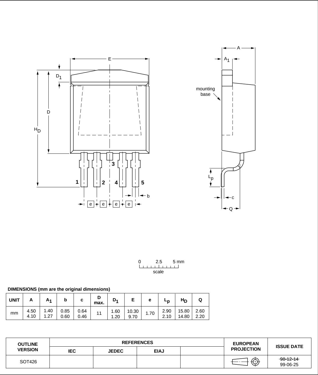
Fig.34. SOT426 surface mounting package 1 , centre pin connected to mounting base.
