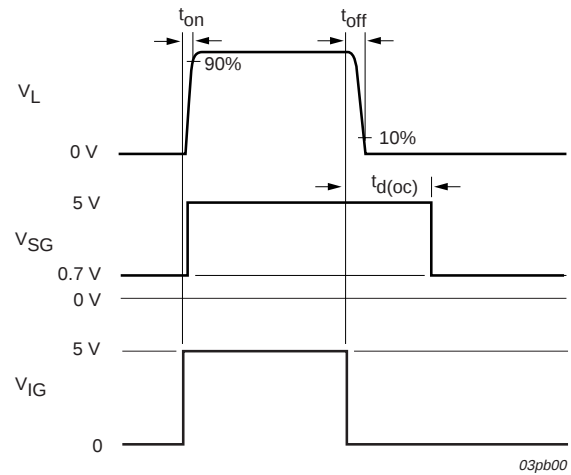
Fig 14. Open circuit detect waveforms.
