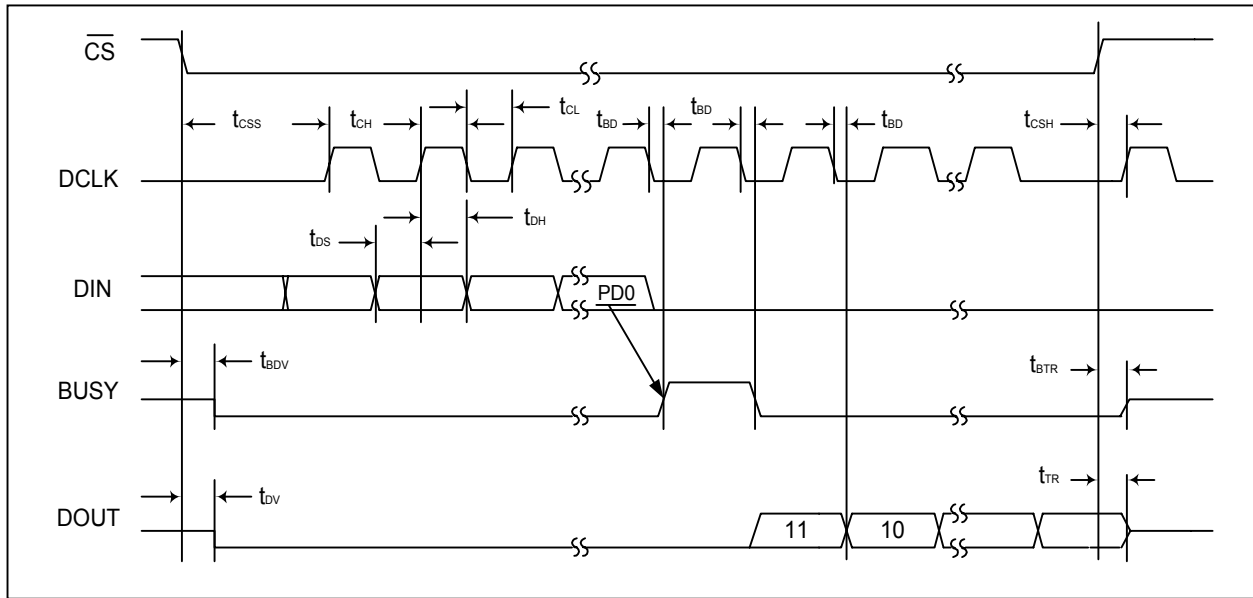
FIGURE 8. Detailed Timing Diagram.
