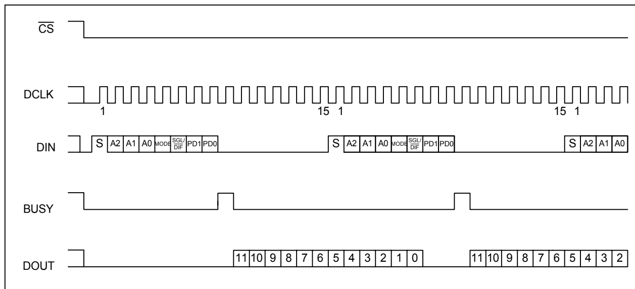
FIGURE 7. Maximum Conversion Rate, 15-Clocks per Conversion.
