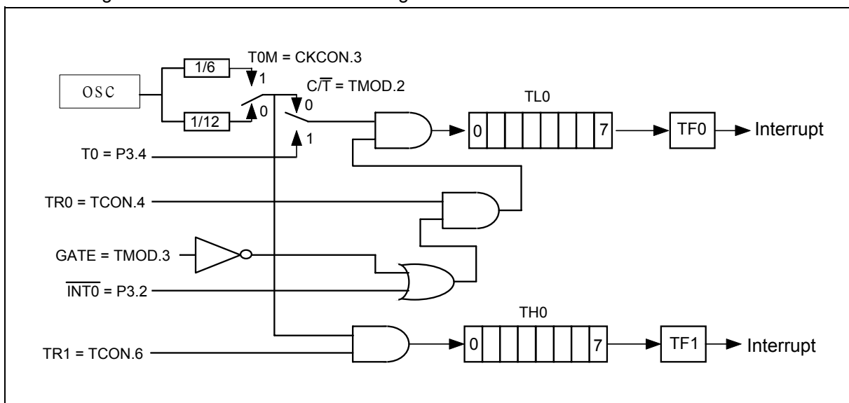
Figure 9-3 Timer/Counter 0 Mode 3
