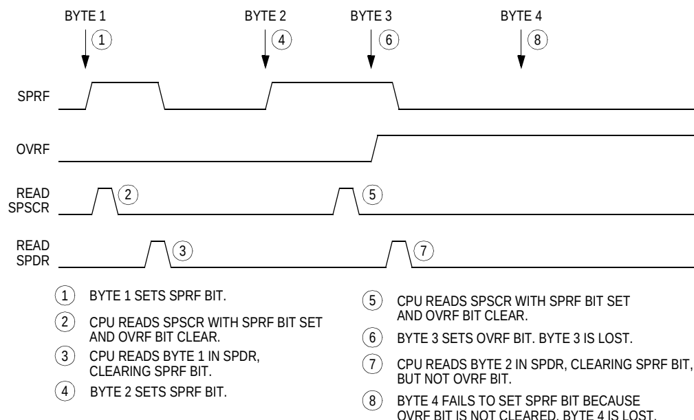
Figure 20-9. Missed Read of Overflow Condition
