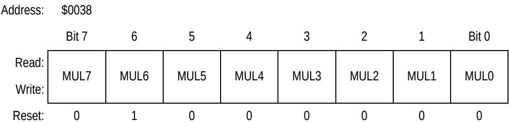
Figure 7-7. PLL Multiplier Select Register Low (PMSL)
