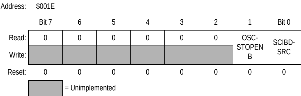
Figure 8-1. Configuration Register 2 (CONFIG2)
