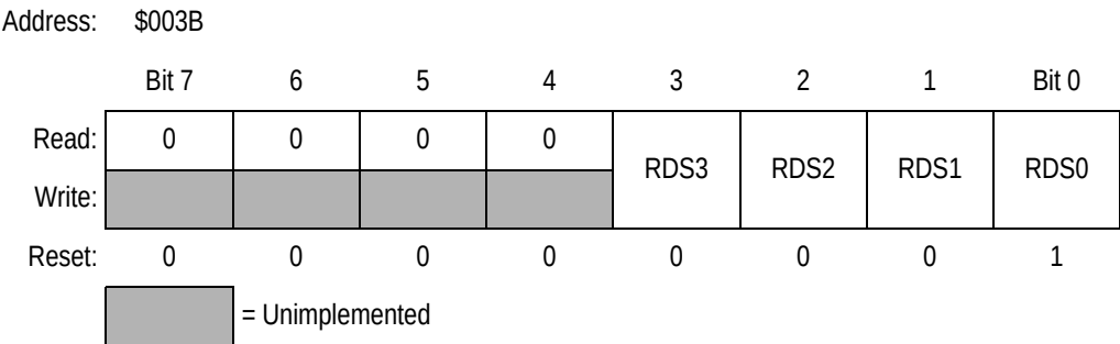
Figure 7-9. PLL Reference Divider Select Register (PMDS)
