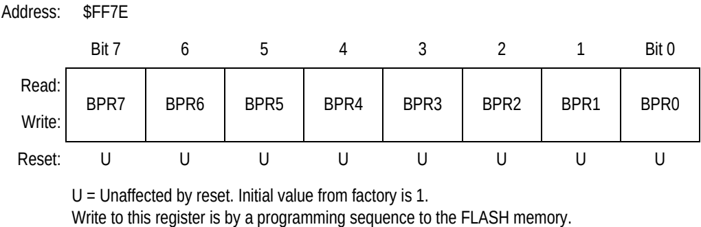
Figure 11-3. FLASH Block Protect Register (FLBPR)
