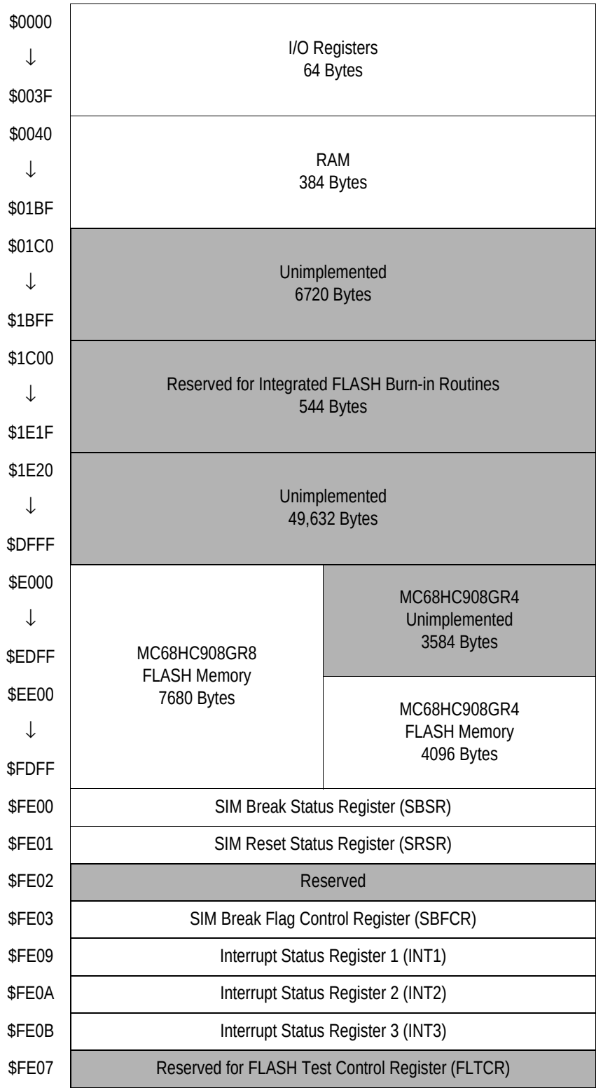
Figure 2-1. Memory Map
