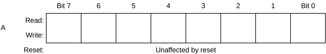
Figure 10-2. Accumulator (A)
