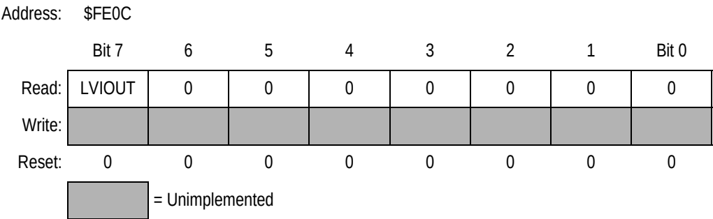
Figure 14-3. LVI Status Register (LVISR)
