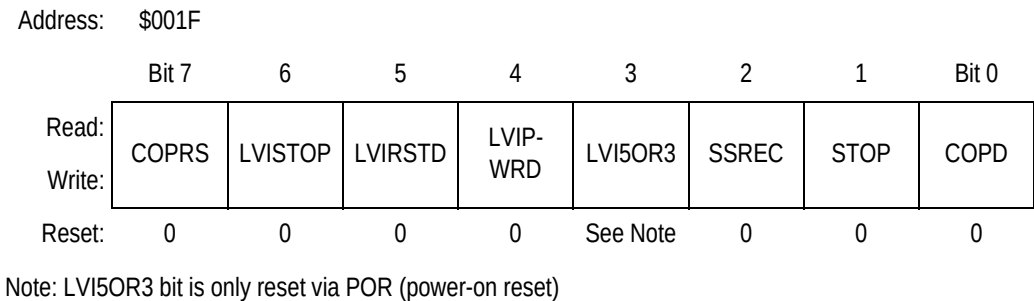
Figure 8-2. Configuration Register 1 (CONFIG1)
