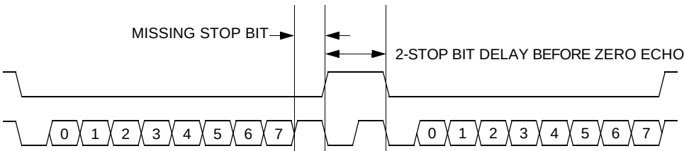
Figure 15-4. Break Transaction
