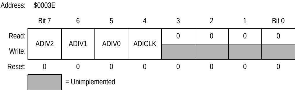
Figure 5-4. ADC Clock Register (ADCLK)
