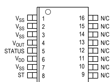
Figure 2. Pin Connections
