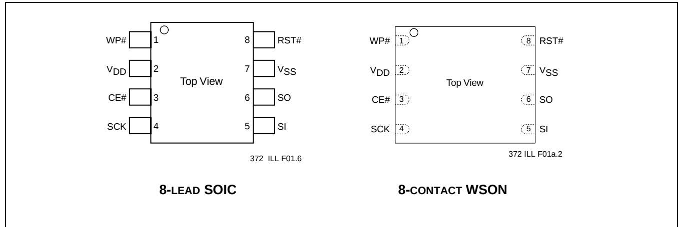
FIGURE 1: PIN ASSIGNMENTS
