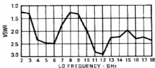
L-Port VSWR @ + 21 dBm
