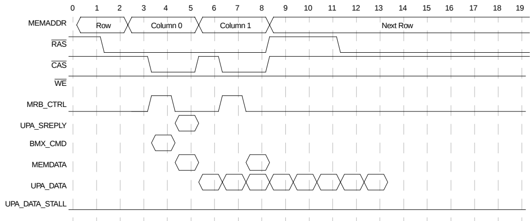
Figure 41. Minimum U2S Read Timing
