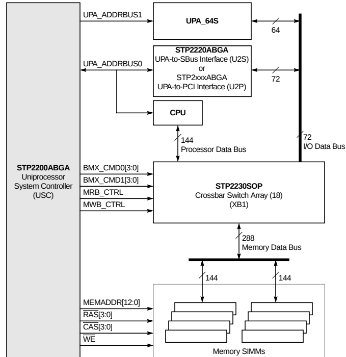
Figure 2. USC Typical Application Diagram
