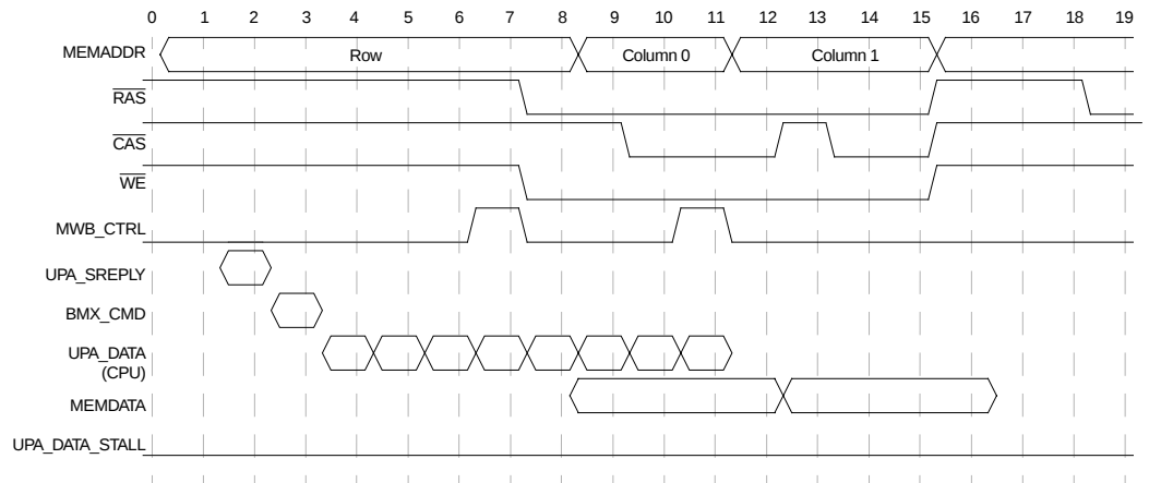
Figure 42. Minimum U2S Write Timing
