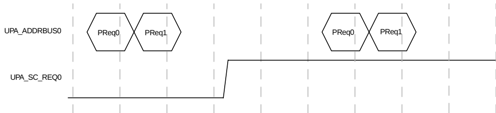
Figure 5. Best-Case PRequest-to-PRequest Timing (ABus0 to ABus0)
