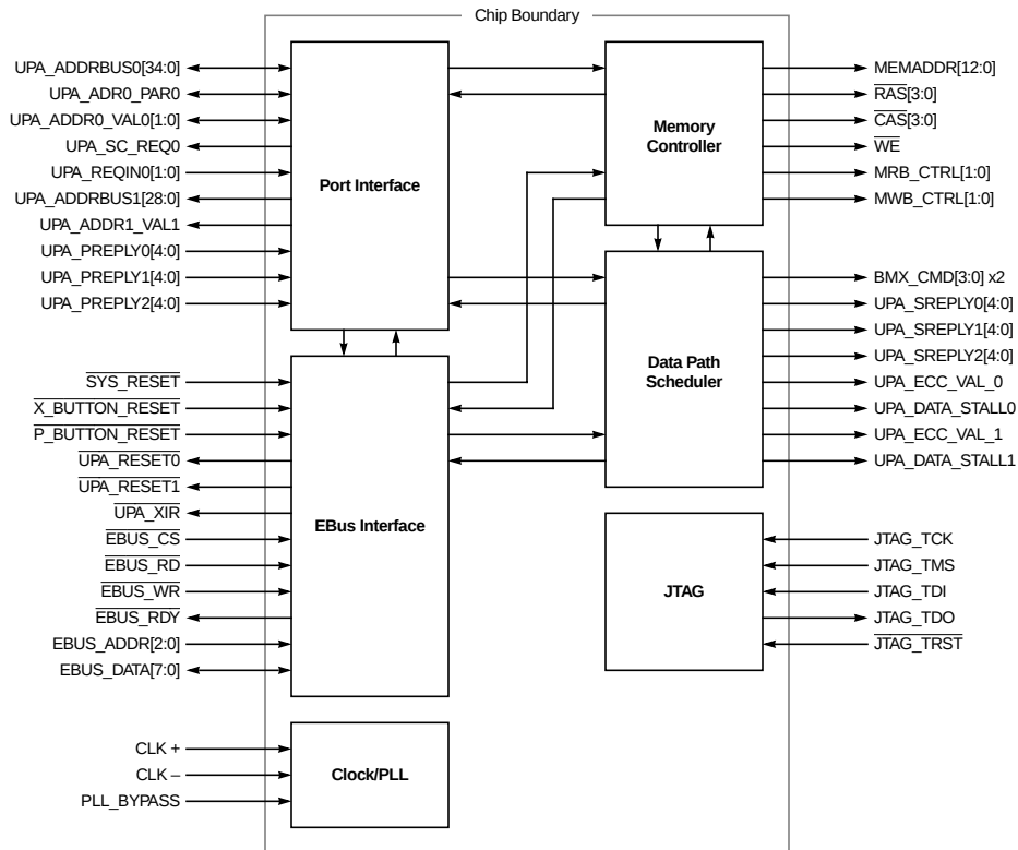
Figure 1. USC Block Diagram
