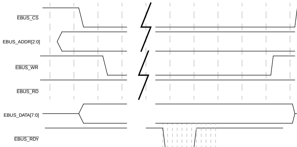
Figure 45. External EBus Write Timing
