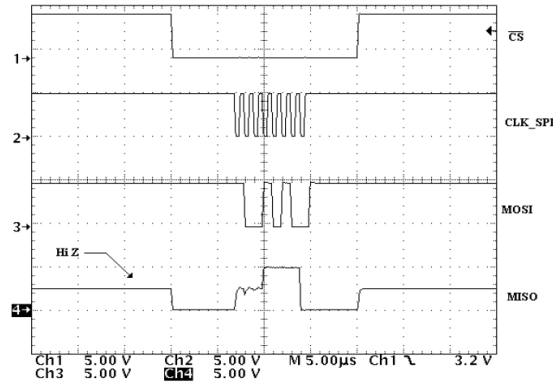
Figure 14. Programming Sequence
