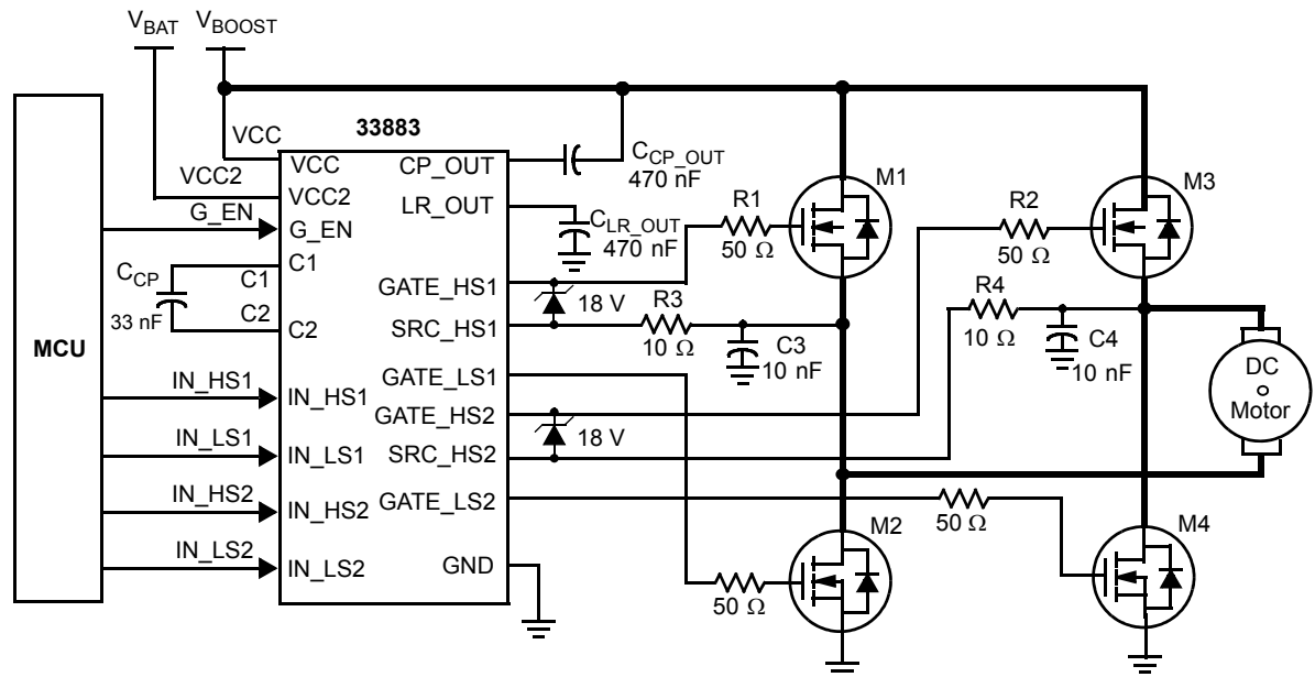
Figure 14. Application Schematic with External Protection Circuit
