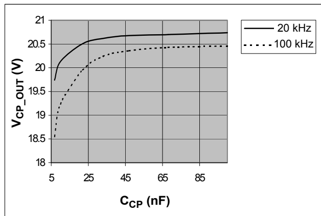
MTP60N06HD ( Q_g = 50 nC)
