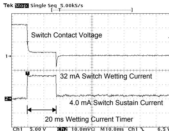
Figure 10. Contact Wetting and Sustain Current for Switch-to-Ground Input
