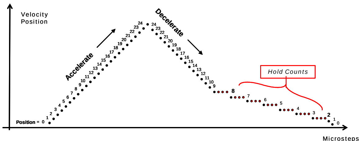
Figure 9. Deceleration Ramp
