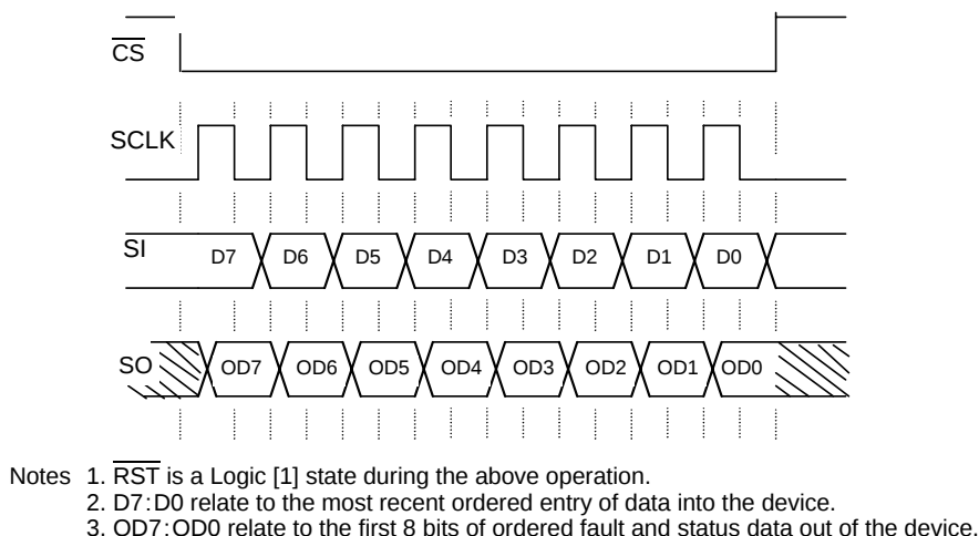
Figure 9. Single 8-Bit Word SPI Communication
