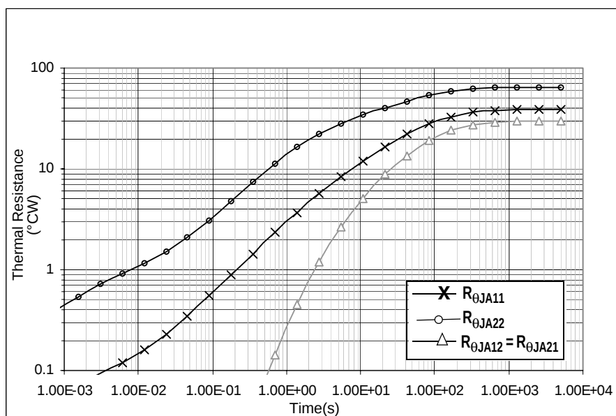
Figure 15. Transient Thermal Resistance R_{\theta JA} (1.0 W Step Response) Device on Thermal Test Board Area A = 600 (mm²)
