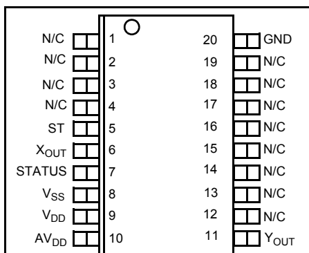
Figure 2. Pin Connections
