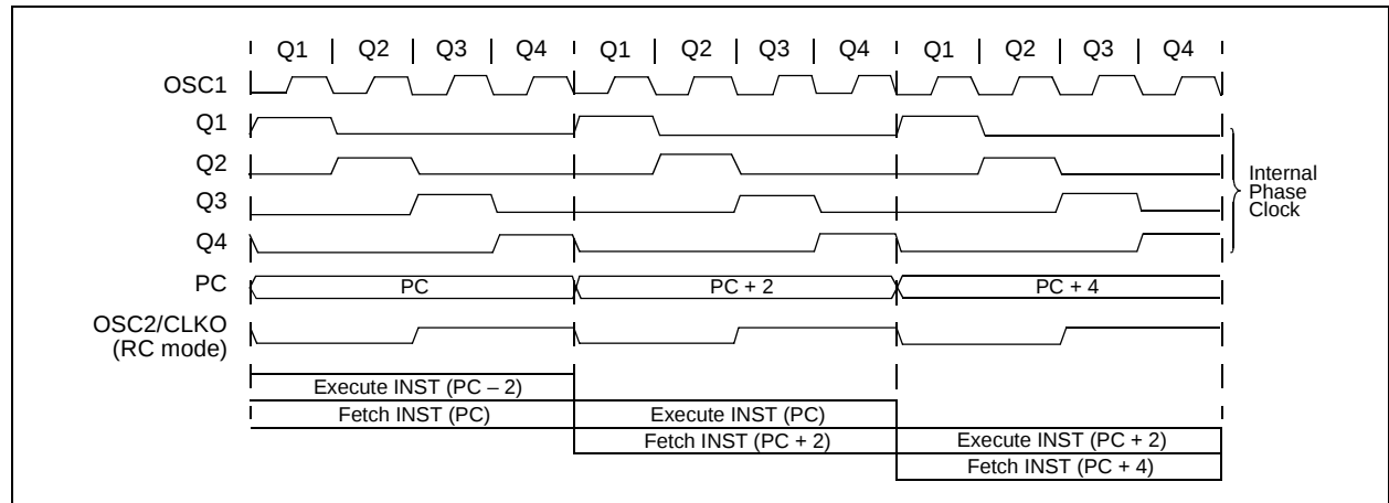
FIGURE 5-4: CLOCK/INSTRUCTION CYCLE
