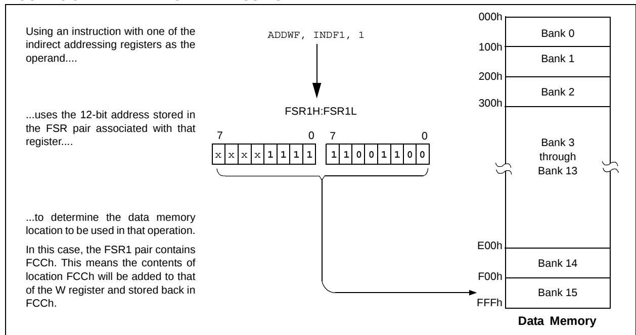
FIGURE 5-8: INDIRECT ADDRESSING
