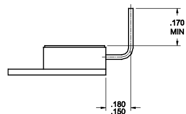
Up Leads (UB Suffix)
