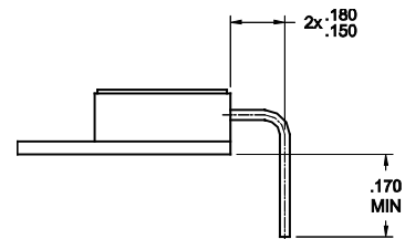
Bent Down Leads (DB Suffix)
