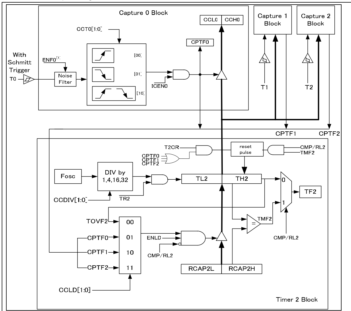
Timer2/capture modules
