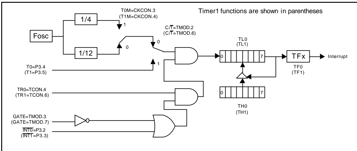
Figure 12-2: Timer/Counter 0 & 1 in Mode 2
