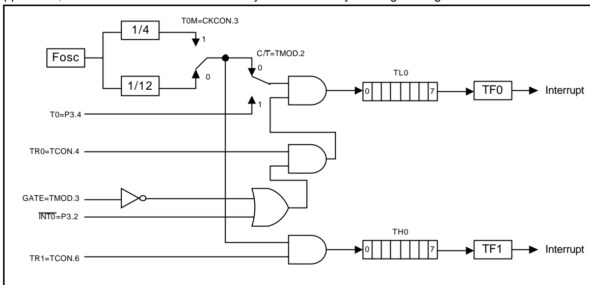
Figure 12-3: Timer/Counter Mode 3
