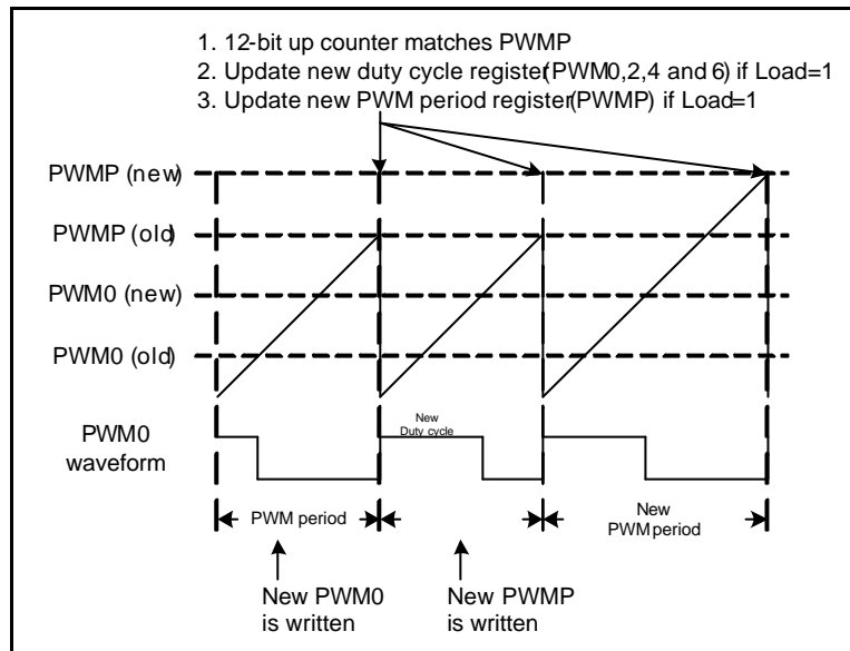
Figure 14-16: Edge-Aligned PWM
