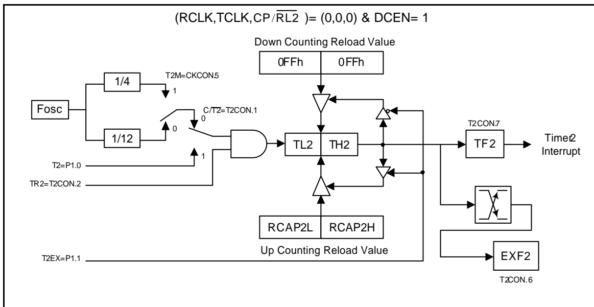
Figure 12-6: 16-Bit Auto-reload Up/Down Counter
