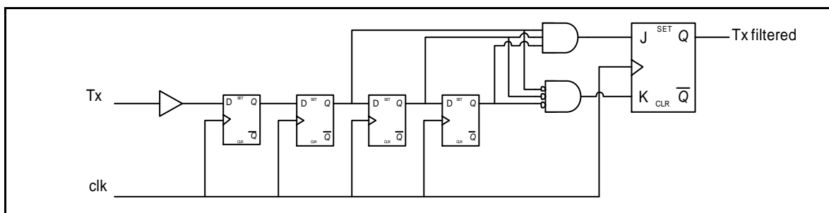
Figure 15-1: Noise Filter
