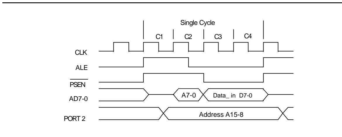
Figure 8-1: Single Cycle Instruction Timing
