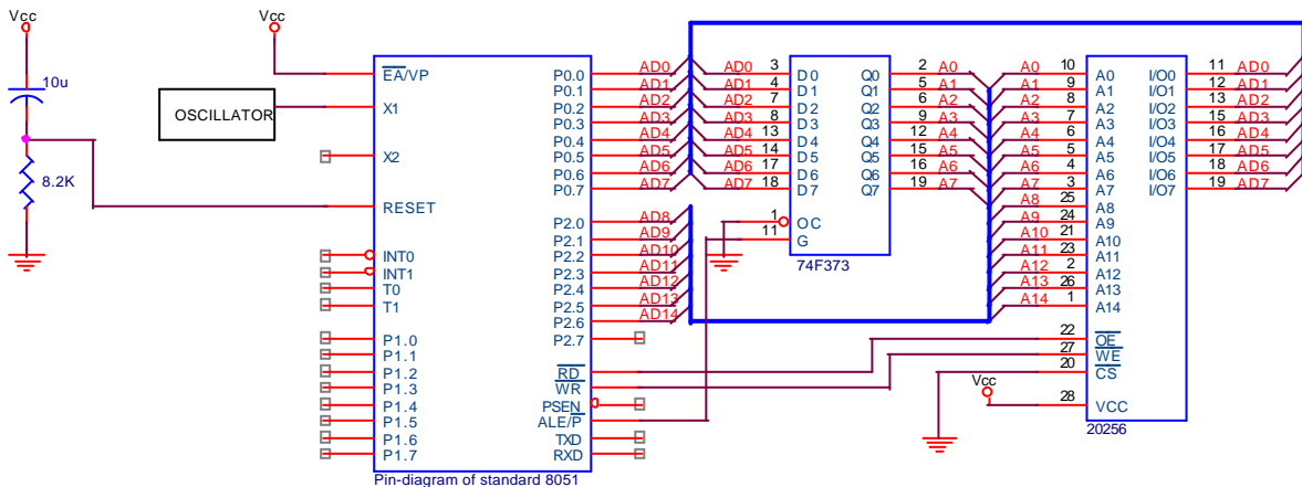
Figure 26-2: Typical External Data Memory and Oscillator connections
