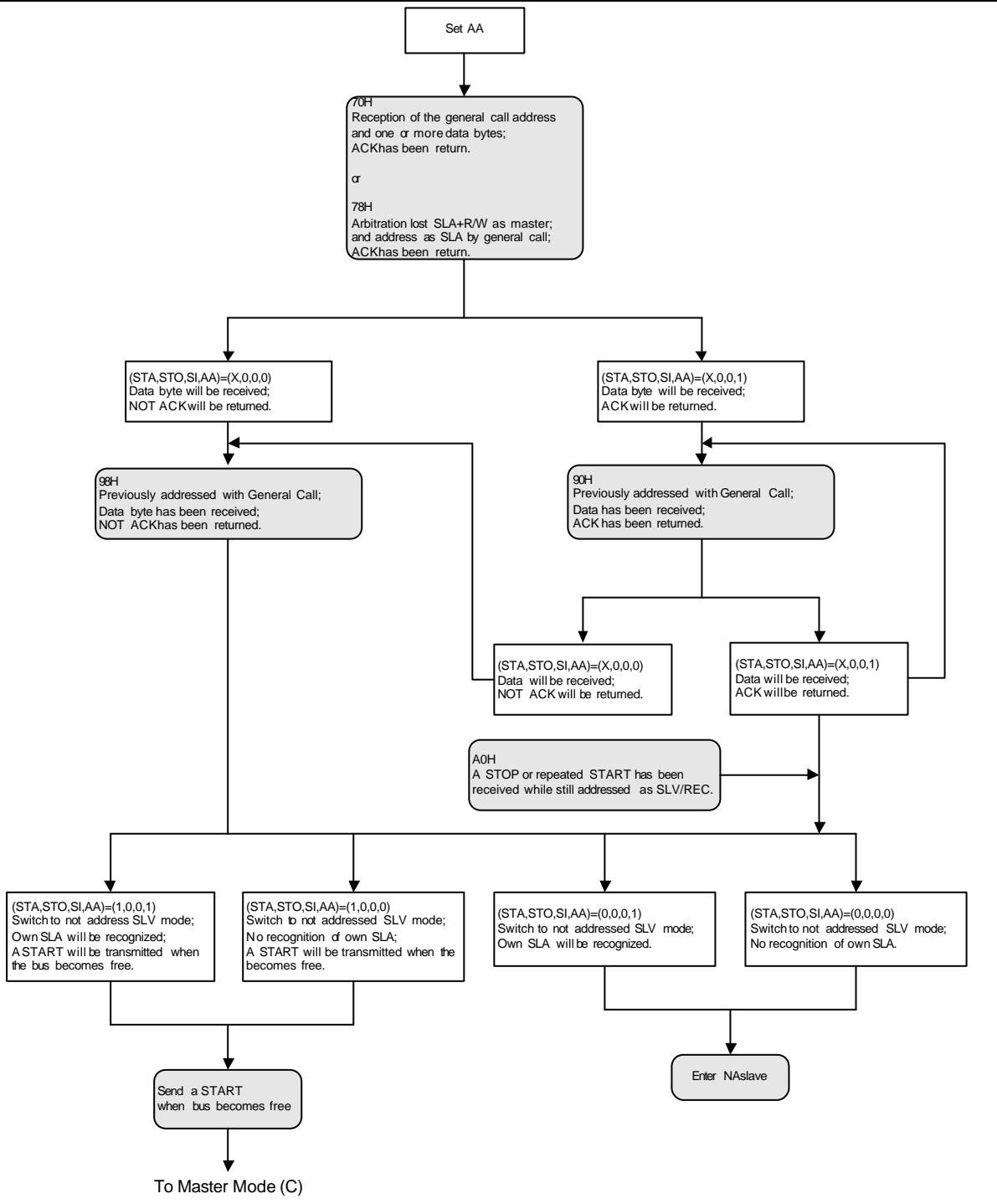
Figure 17-8: General Call Address
