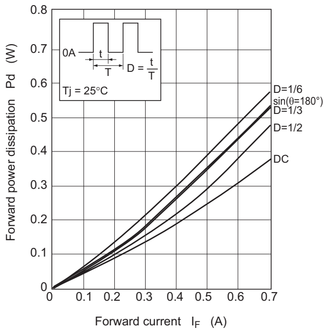
Fig.4 Forward power dissipation vs. Forward current
