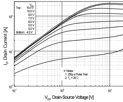
Figure 1. On-Region Characteristics
