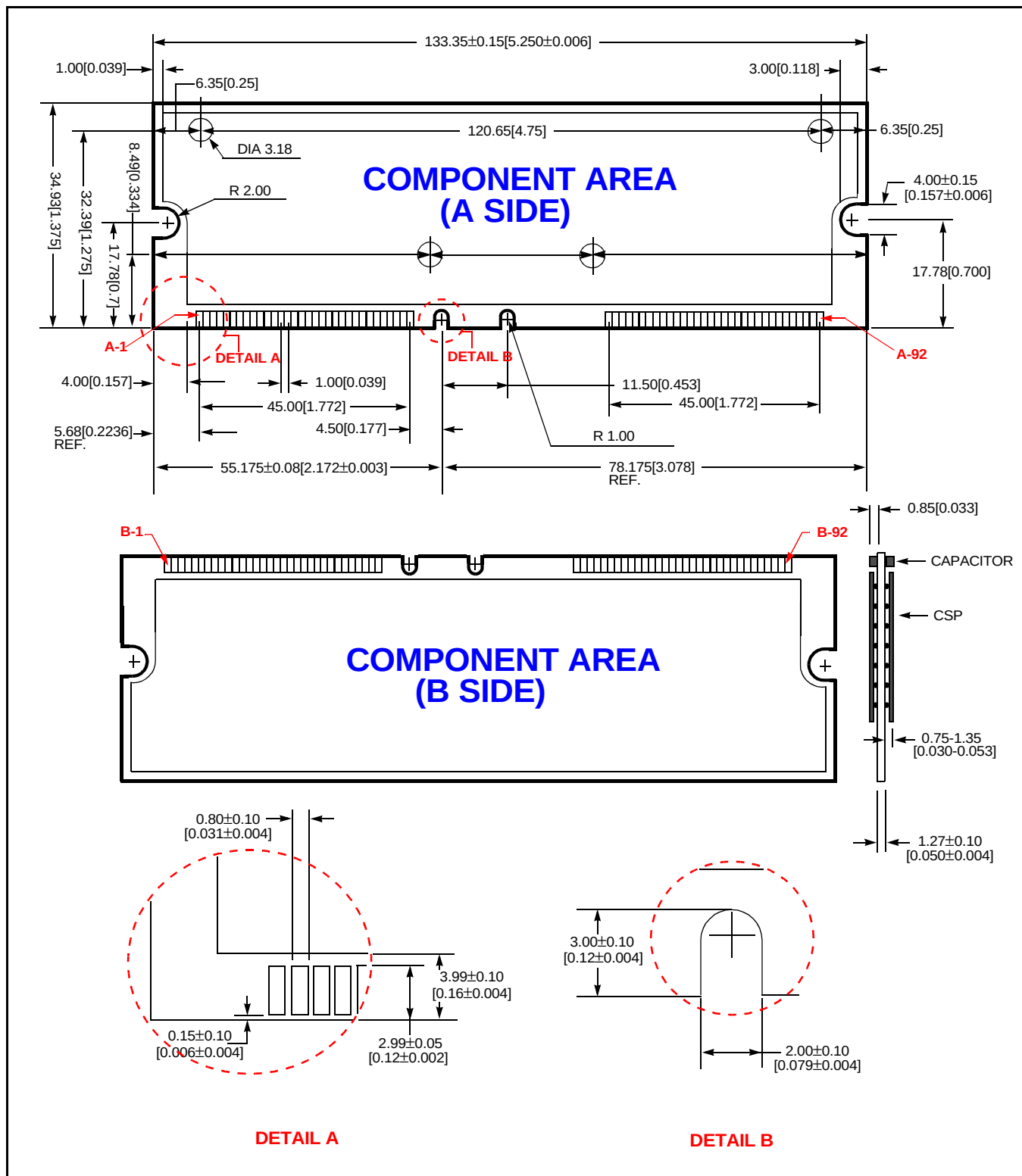
Figure 3: RIMM Module PCB Physical Dimensions
