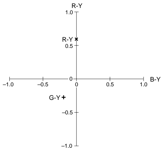
COL_AXIS = 1 (PAL/SECAM)
