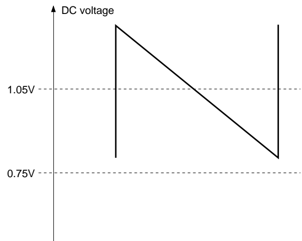
Abnormal input to VPROT input pin example 2 (The bottom edge of the input signal does not fall to 0.75V or less.)
