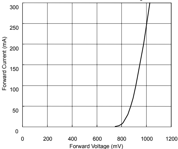
ZD5240B Forward Current vs Forward Voltage
