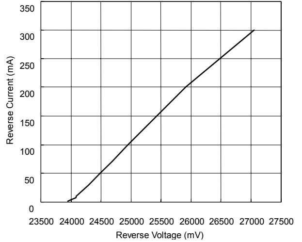
ZD5252B Reverse Current vs Reverse Voltage
