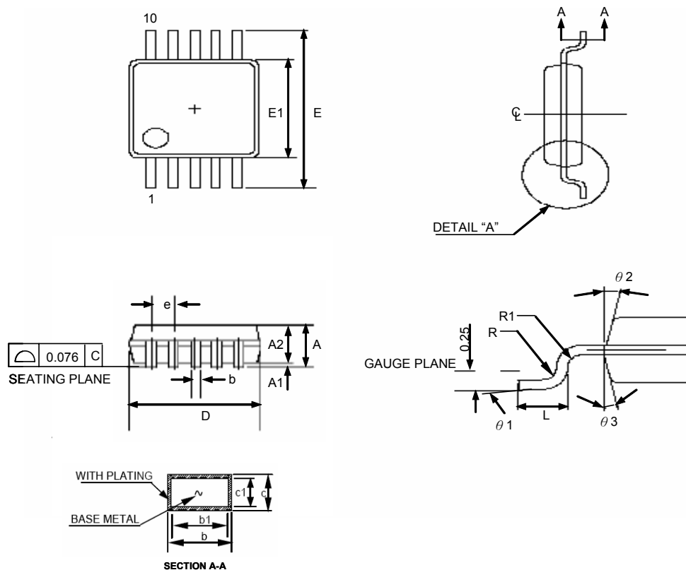
MSOP-10 Package
