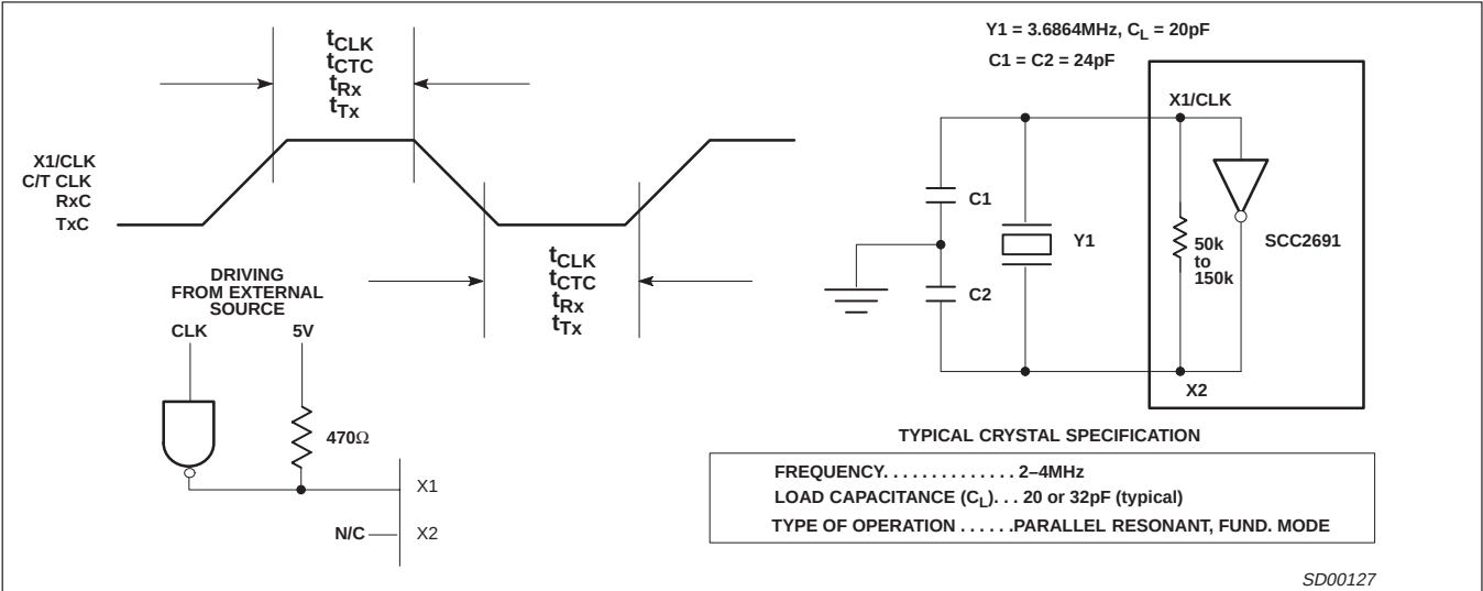
Figure 7. Clock Timing
