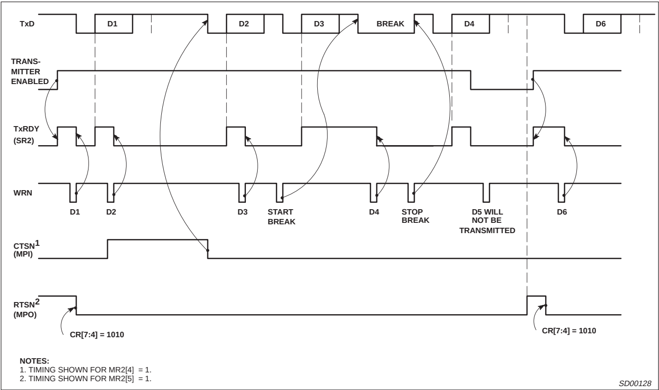
Figure 10. Transmitter Timing
