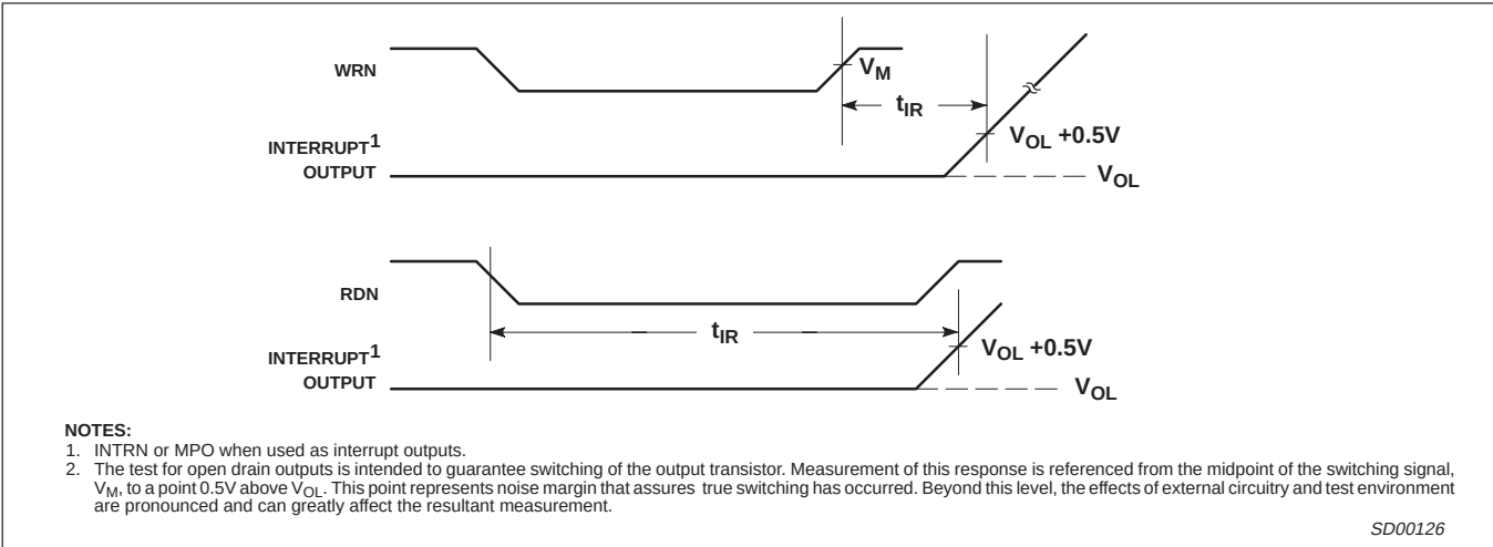
Figure 6. Interrupt Timing
