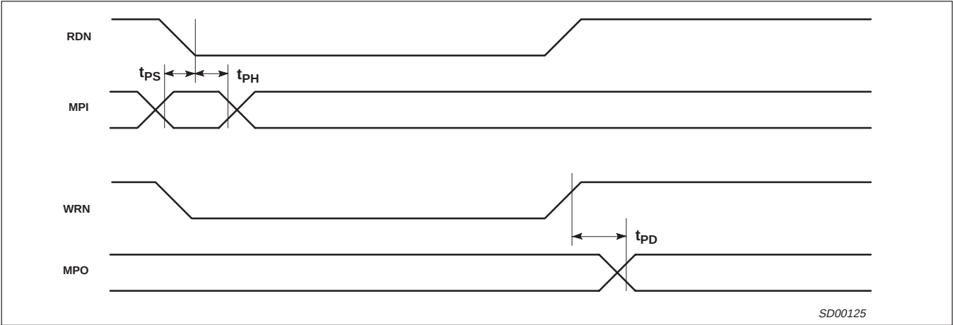
Figure 5. I/O Timing
