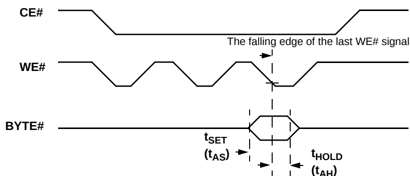
Figure 19. BYTE# Timing for Write Operations
