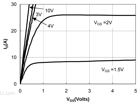
Figure 1: On-Regions CharacteristicCS
