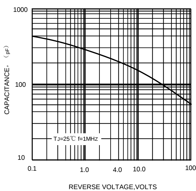
FIG.4-TYPICAL JUNCTION CAPACITANCE
