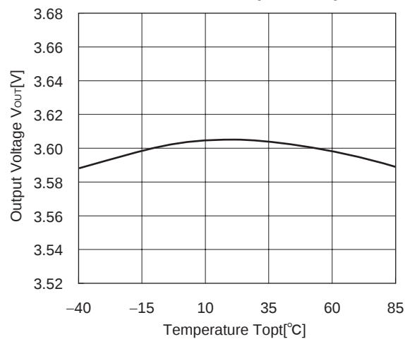
R1180x361x ( V_{IN}=4.6V )
