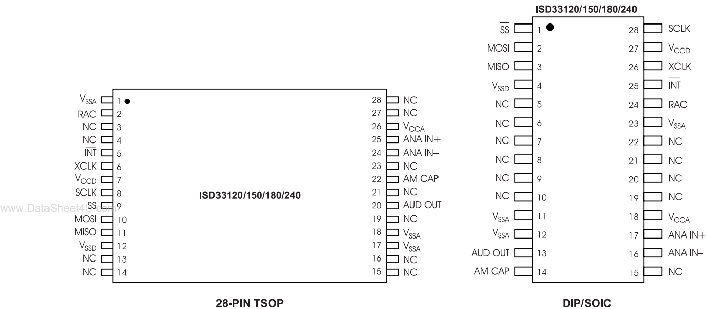
Figure 1: ISD33000 TSOP and DIP/SOIC Pinouts
