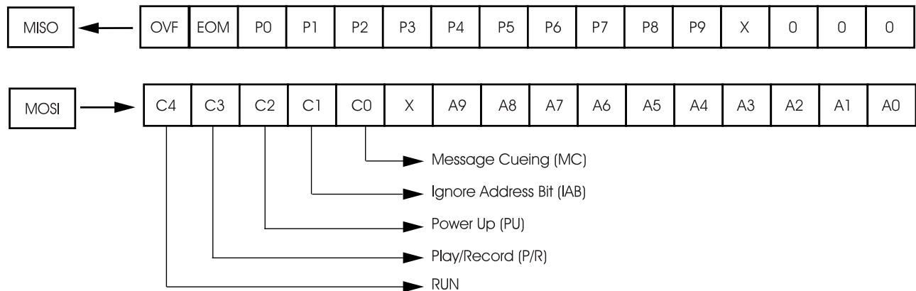
Figure 3: SPI Port
