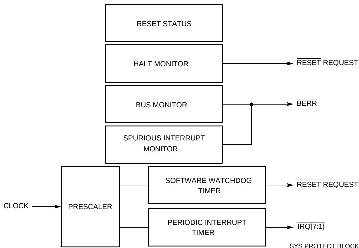
Figure 4-7 System Protection
