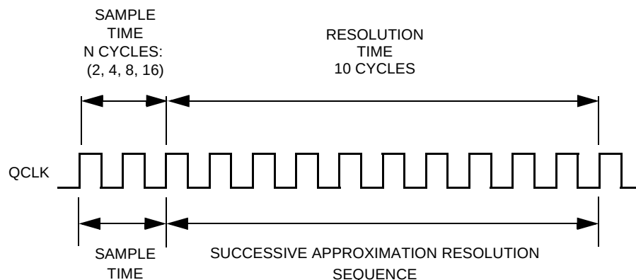
Figure 5-6 Bypass Mode Conversion Timing
