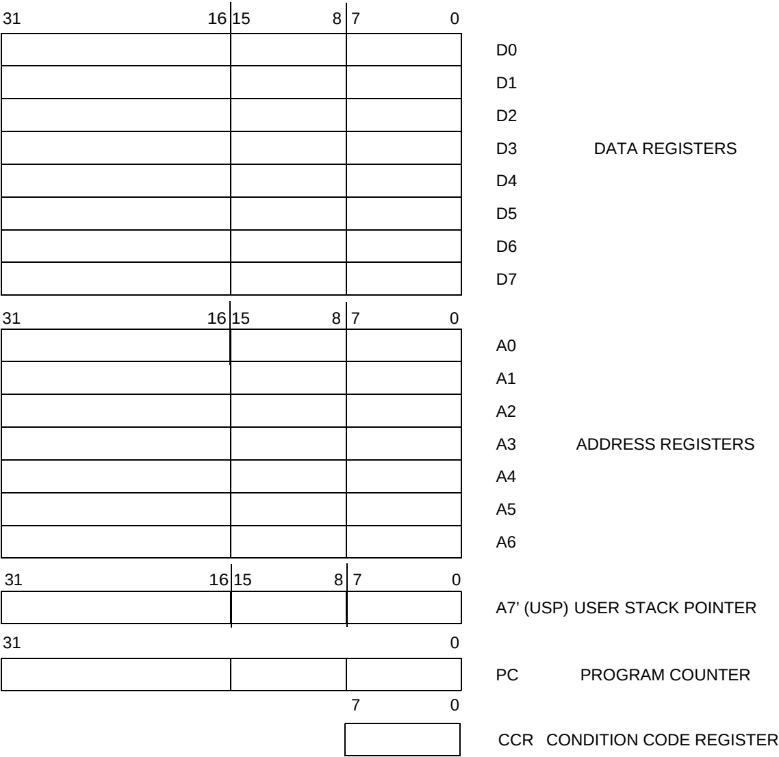
CPU32 USER PROG MODEL
