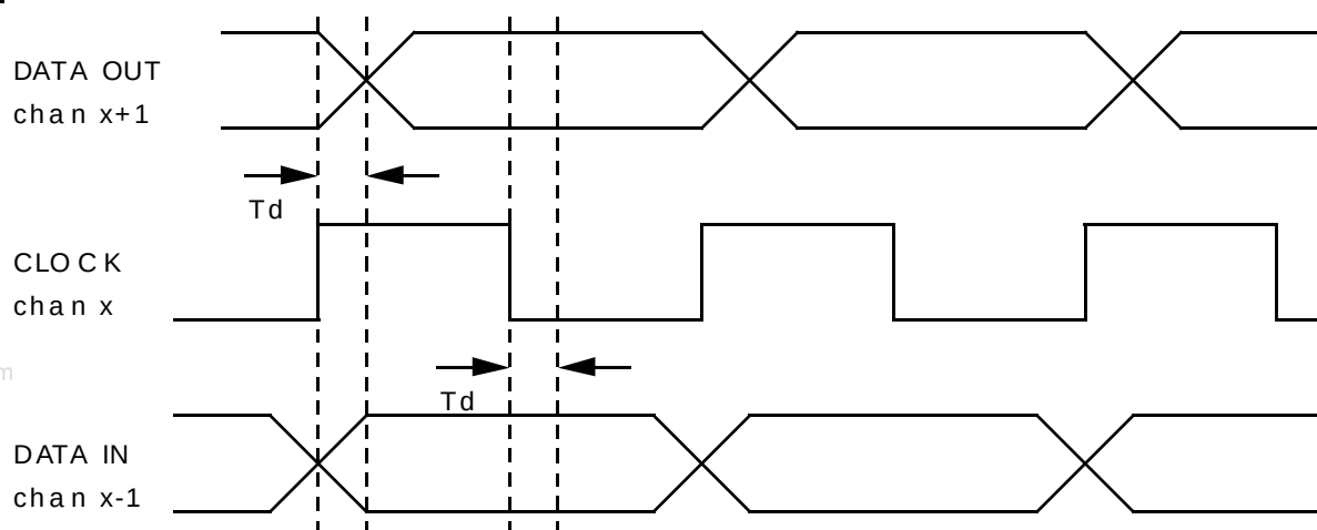
Figure D-29 SIOF Function Data Transition Example
