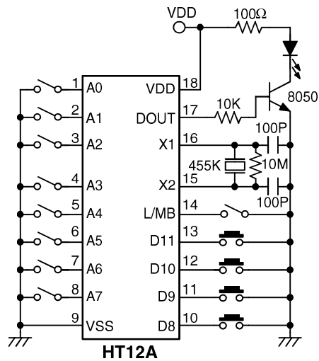
Application circuit 1
