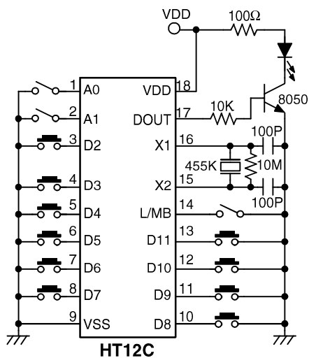
Application circuit 3
