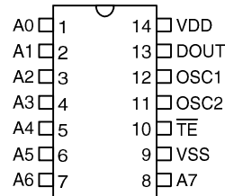
HT12E - 14 DIP
