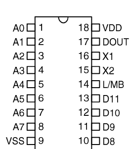
HT12B -18 DIP
