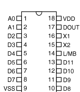
HT12C -18 DIP
