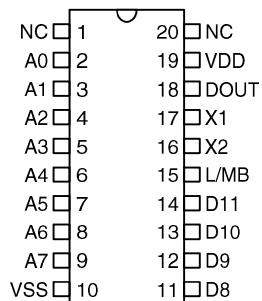
HT12B -20 SOP
