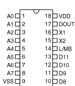
HT12A -18 DIP
