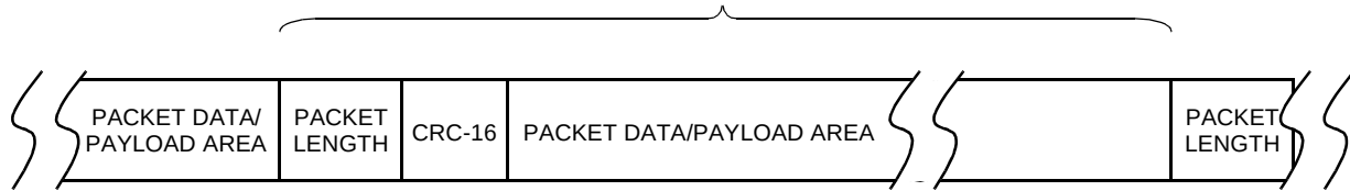
A. GFP encapsulation of packet data without CRC (GFP mode)
