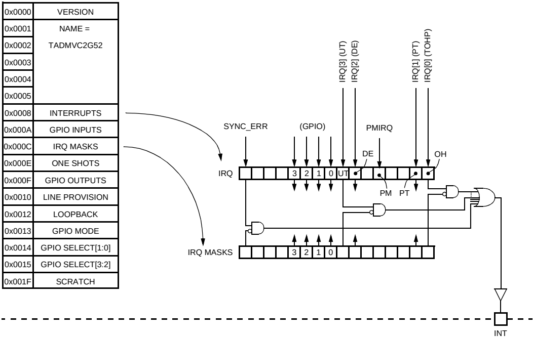
Figure 16. Interrupt Functionality
