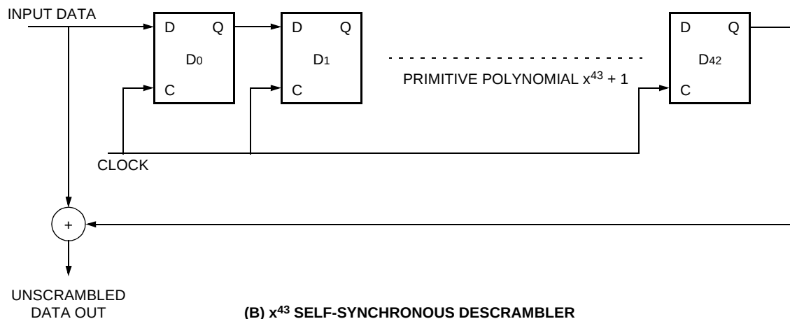
Figure 90. x^{43} Self-Synchronous Scrambler/Descrambler
