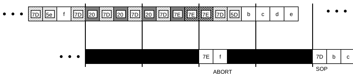
Figure 72. Aborting a Dry
