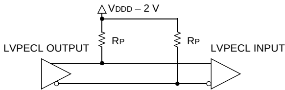
DIFFERENTIAL CONFIGURATION WITH PARALLEL TERMINATION
