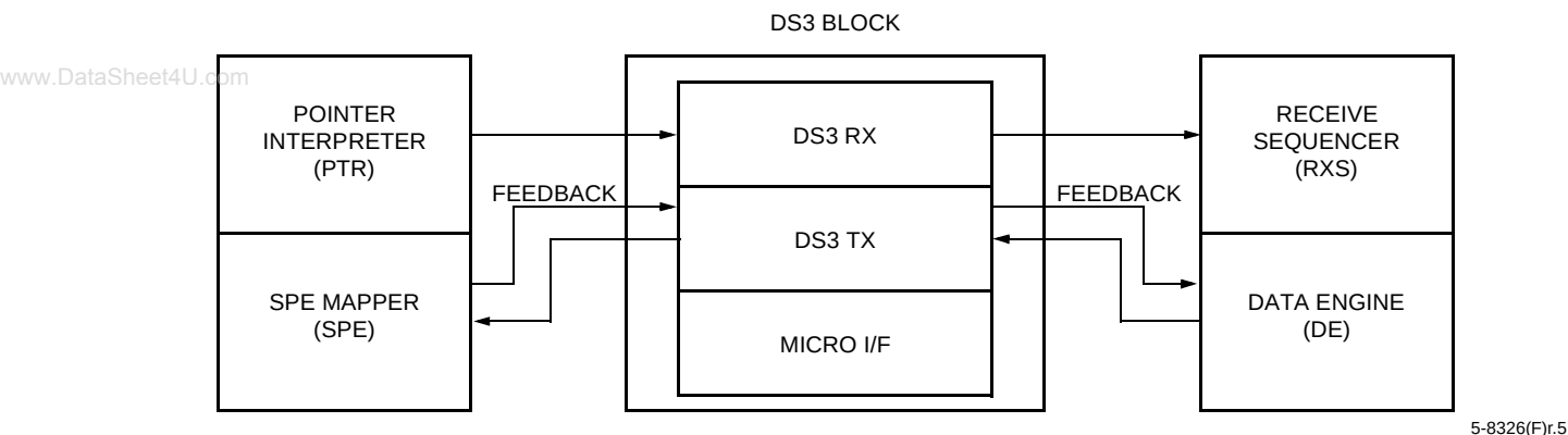
Figure 55. DS3 Block Interface Diagram
