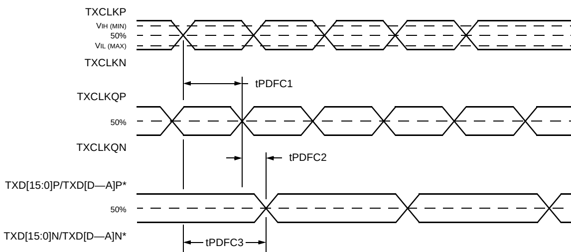
Figure 23. Transmit Line-Side Timing Waveform—OC-48 Forward Clocking
