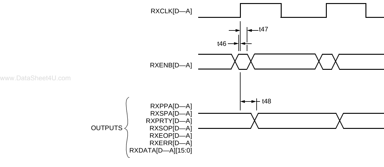
Figure 109. Receive UTOPIA Interface Timing
