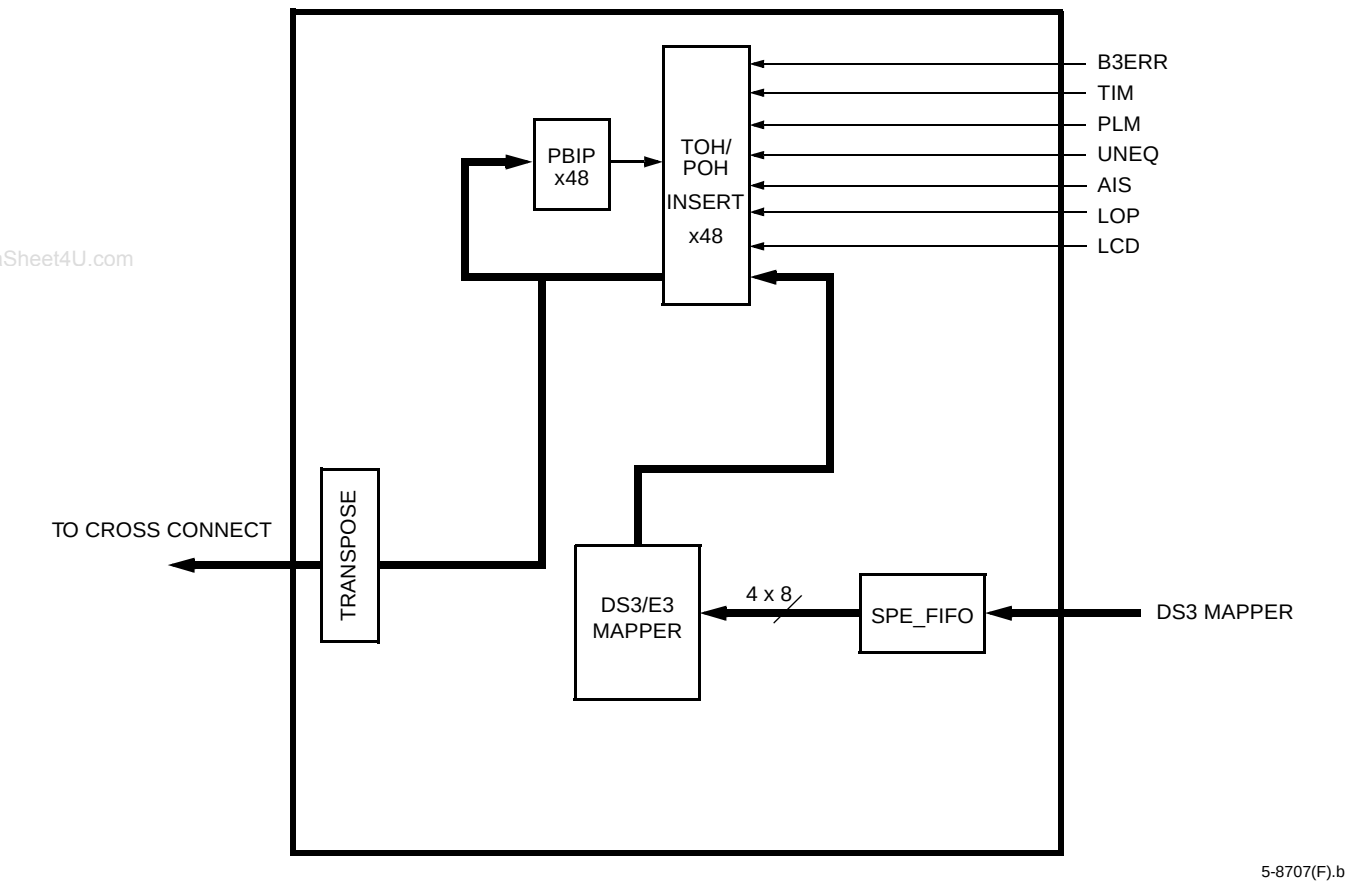
Figure 39. Block Diagram of SPE Mapper Block
