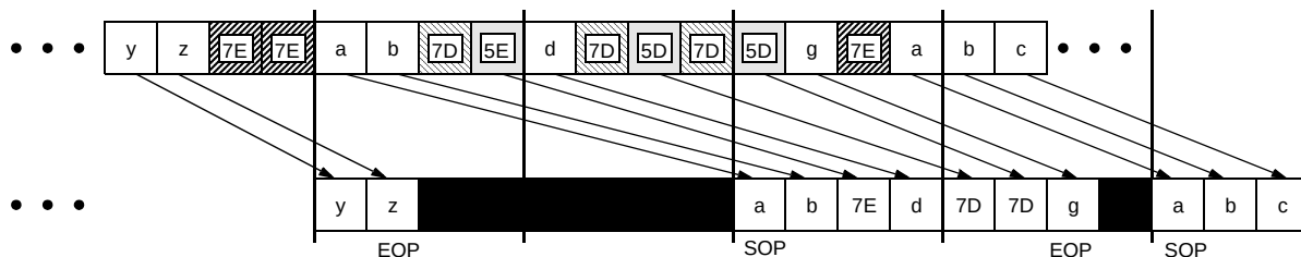
Figure 70. Framing and EOP
