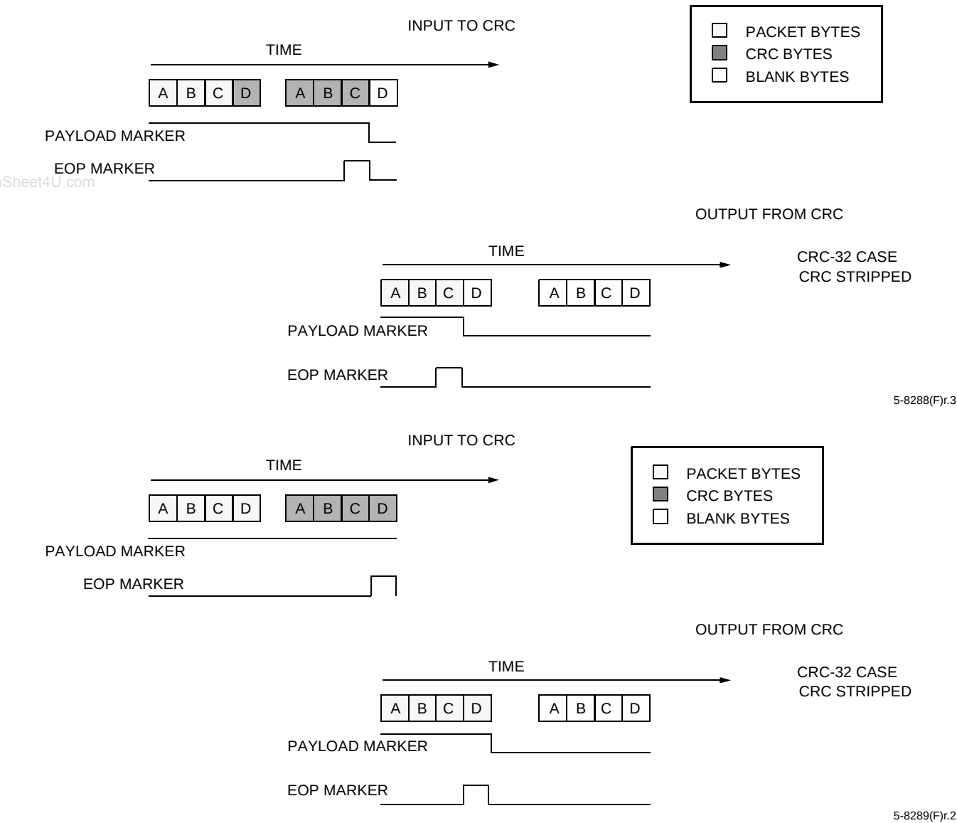
Figure 85. Assorted CRC Checker Cases
