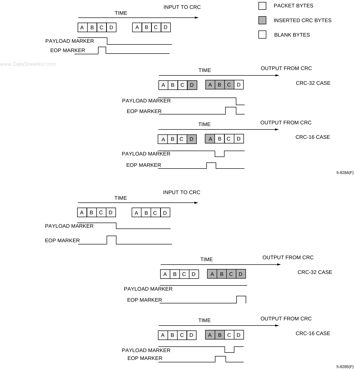
Figure 83. Assorted CRC Generator Cases
