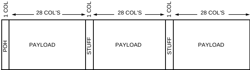
Figure 40. Direct Mapping into STS SPE
