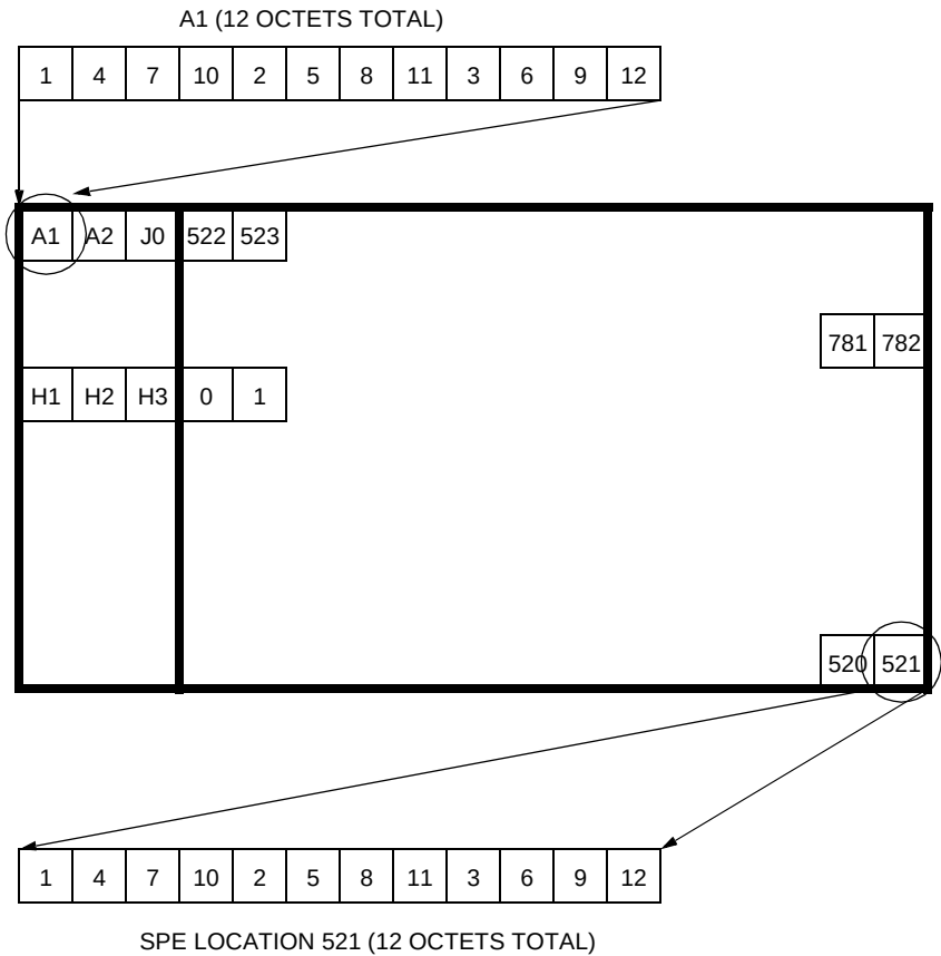
Figure 45. STS-12 Frame Structure
