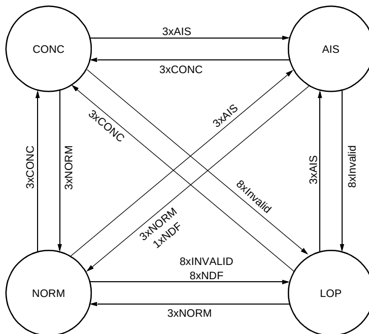
Figure 48. Interpreter State Machine
