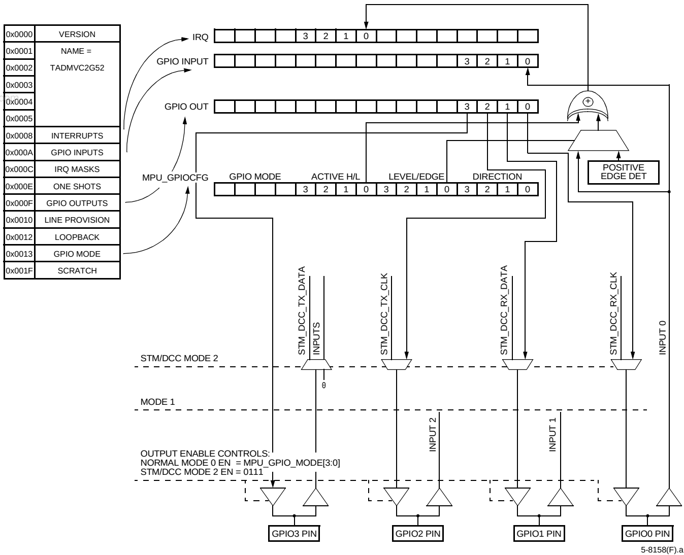
Figure 15. General Input/Output (GPIO)
