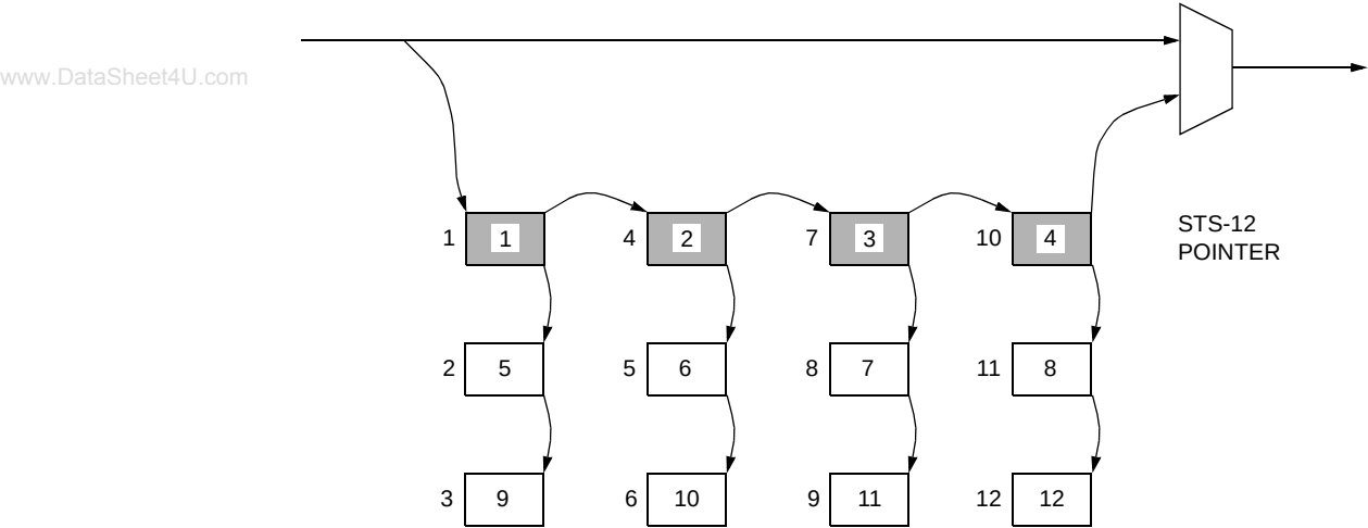
Figure 49. STS-12 RXT Concatenated Offset Passing
