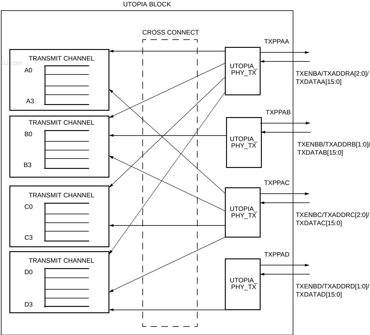
Figure 98. Overall Structure for Transmit Direction
