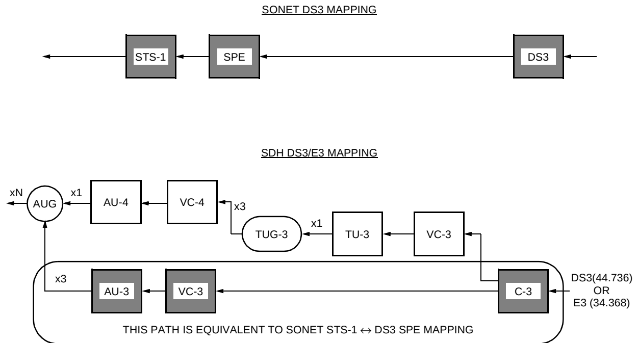
Figure 57. DS3/E3 Mappings
