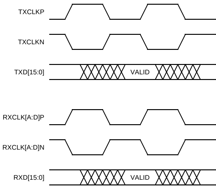
Figure 19. Line Interface
