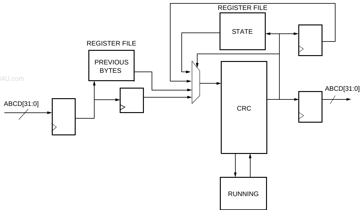
Figure 79. A CRC-16/32 Checker Circuit
