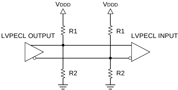
DIFFERENTIAL CONFIGURATION WITH THEVENIN TERMINATION
