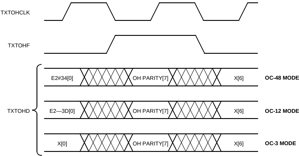
Figure 30. TTOH Interface
