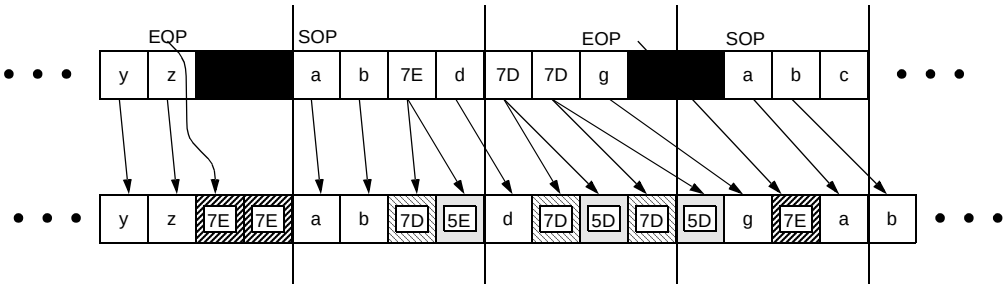
Figure 67. Escaping and EOP
