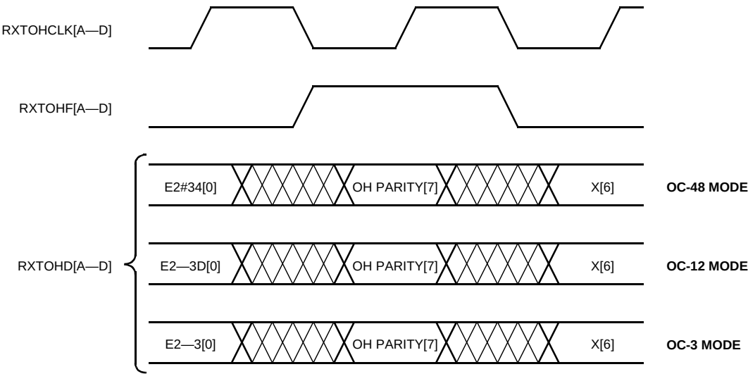
Figure 29. RTOH Interface
