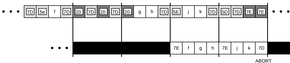
Figure 71. Framing Dry and Abort
