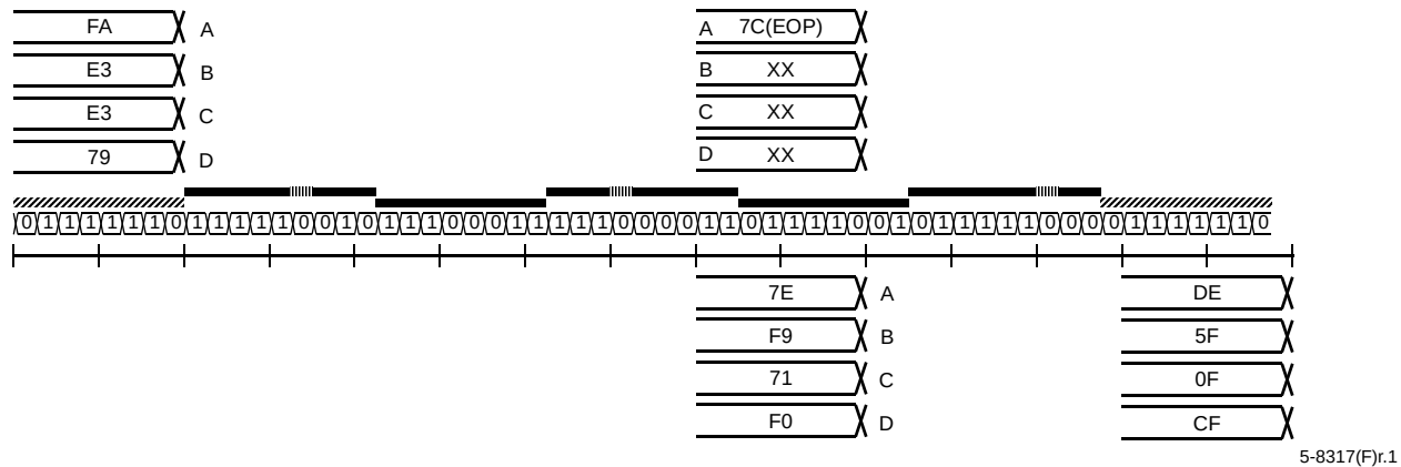
Figure 75. Bit-Synchronous HDLC Escaper Operation
