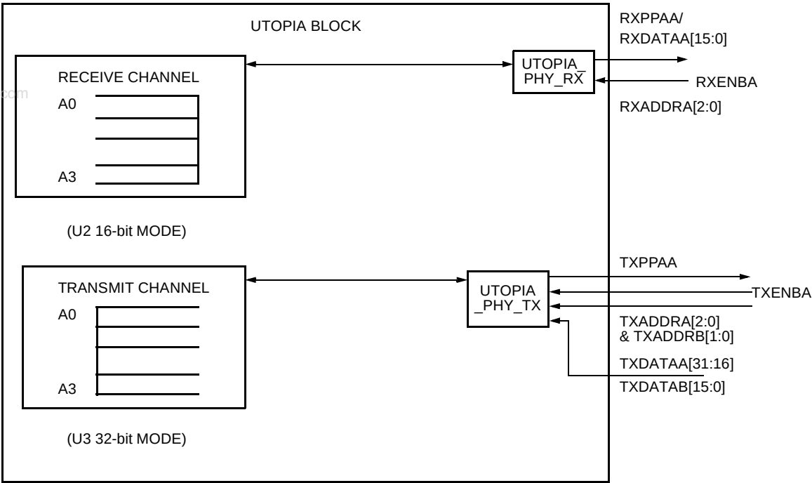
Figure 106. Mixed Modes of Operation of the Receive Side and the Transmit Side
