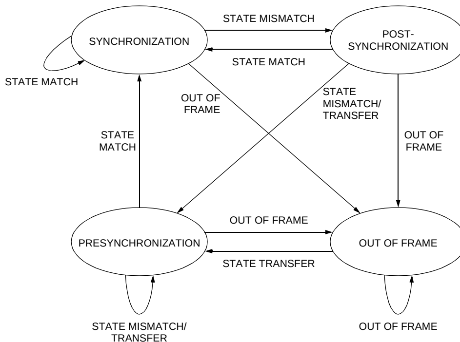
Figure 92. X 48 Scrambler Synchronization State Machine
