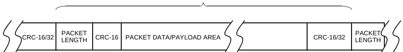
B. GFP encapsulation of information with CRC (GFP-CRC mode)
