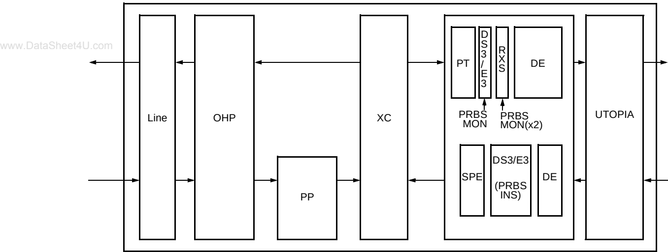
Figure 63. MARS2G5 P-Pro PRBS Monitor/Generator Locations
