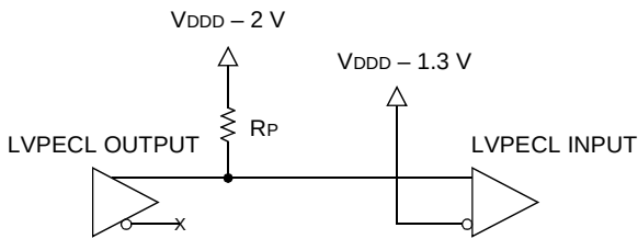
SINGLE-ENDED CONFIGURATION WITH PARALLEL TERMINATION
