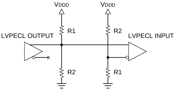
SINGLE-ENDED CONFIGURATION WITH THEVENIN TERMINATION
