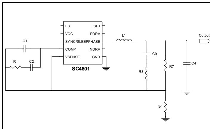
Figure 3. Compensation network provides 3 poles and 2 zeros.
