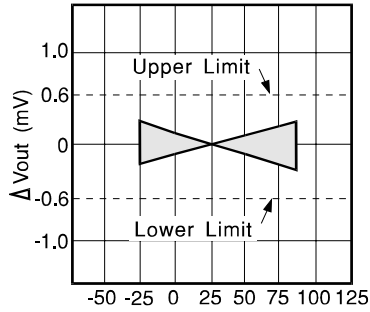
Temperature °C VRE210C
