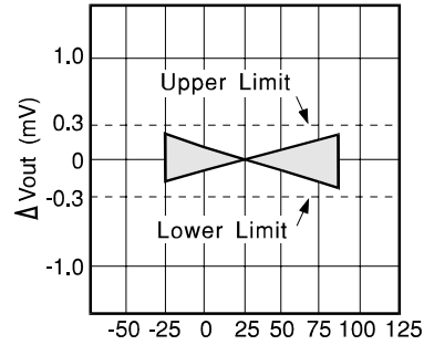
Temperature °C VRE210CA
