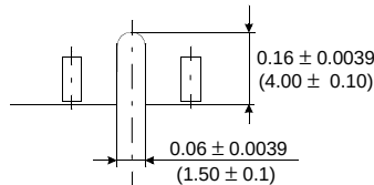
Detail Z
