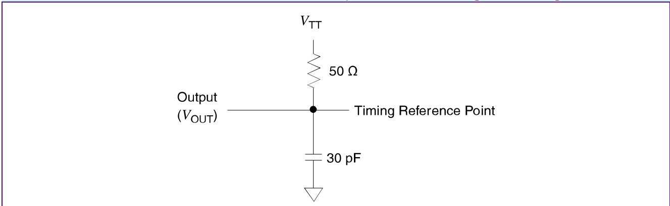
AC Output Load Circuit Diagram / Timing Reference Load
