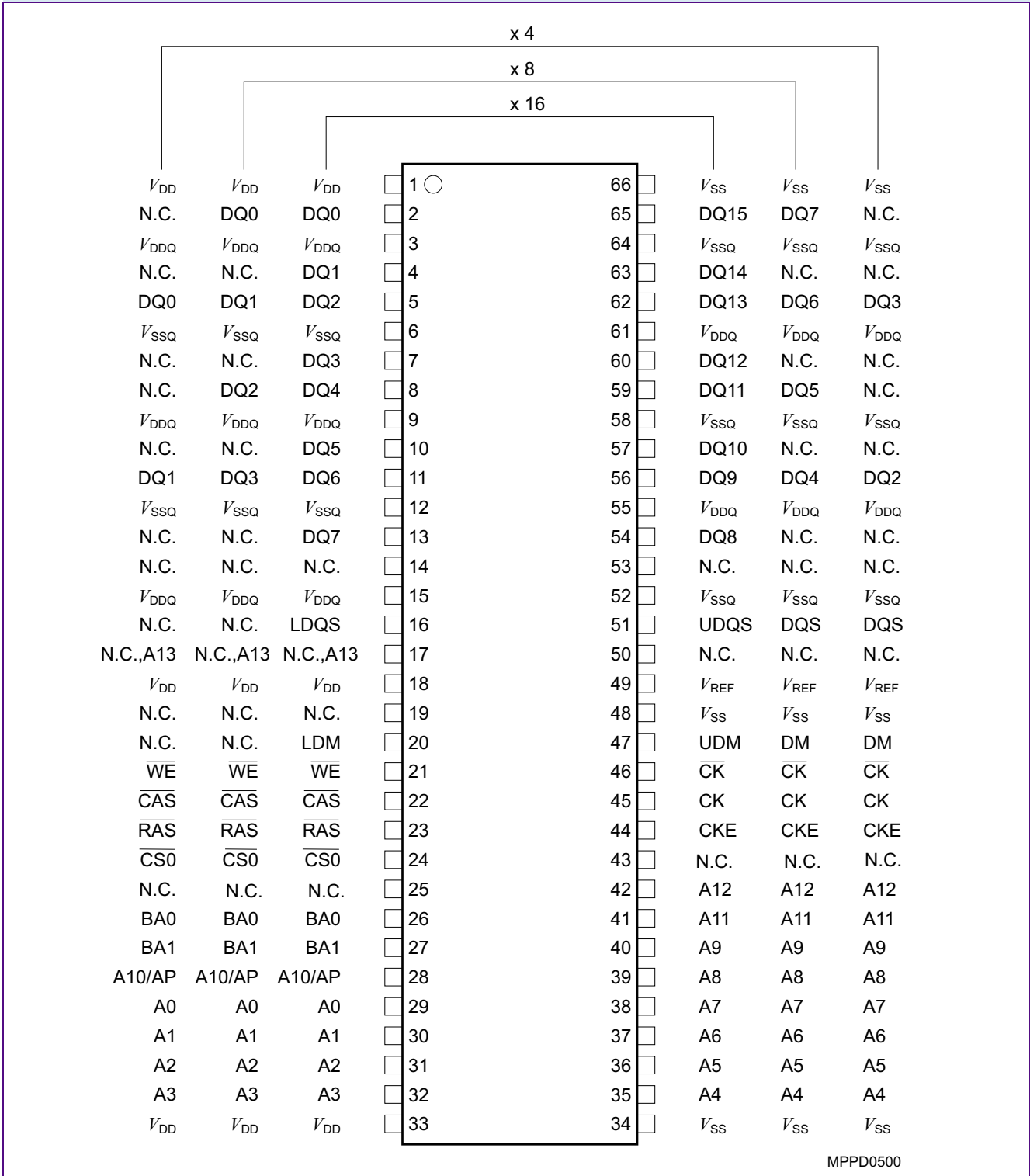
FIGURE 4 Configuration TSOP166, Top View
