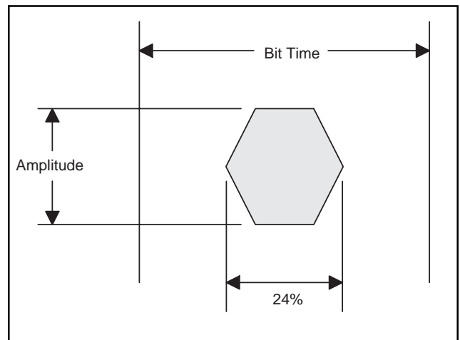
Figure 21. Receiver Input Eye Diagram Jitter Mask
