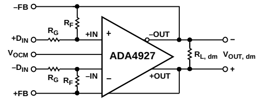
Figure 46. Circuit Definitions
