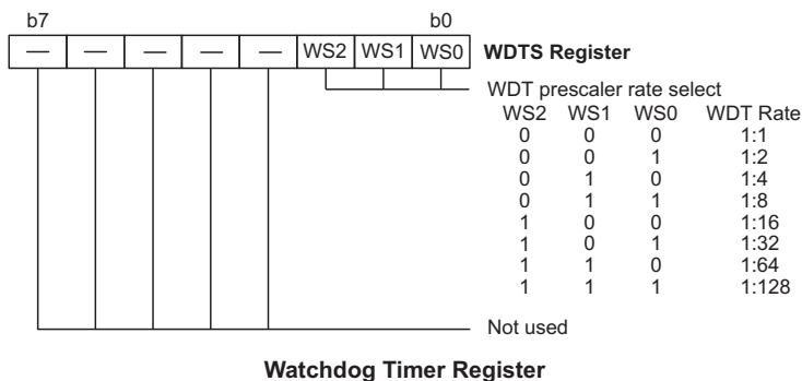
Watchdog Timer Register
