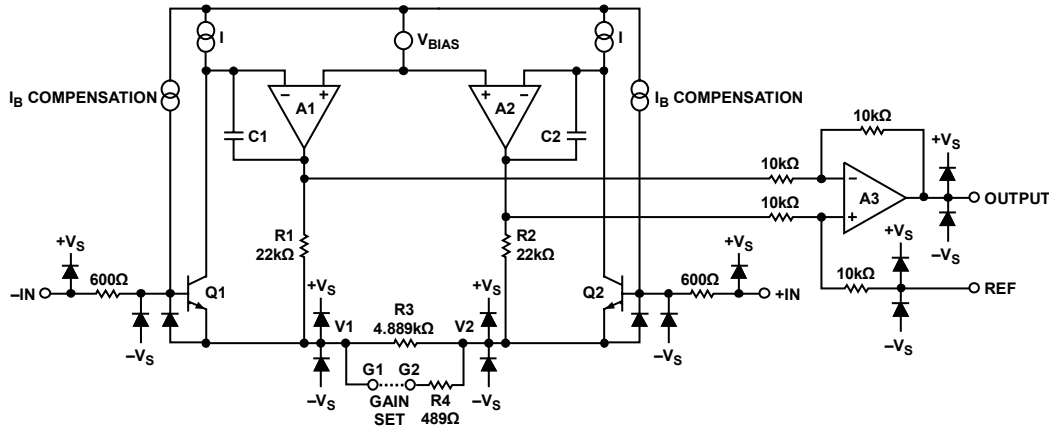
Figure 41. Simplified Schematic
